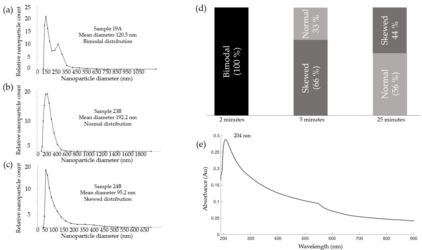
Figure 4. (a) Sample with bimodal nanoparticle size distribution after 2 min; (b) sample with normal nanoparticle size distribution after 5 min; (c) sample with positively skewed nanoparticle size distribution after 25 min; (d) effect of ablation time on nanoparticle size distribution. All samples are bimodal at 2 min, mostly skewed at 5 minutes and mostly normally distributed at 25 min; (e) typical UV–Vis curve for a magnesium colloid. A distinct peak is observed at a wavelength of about 204 nm.
