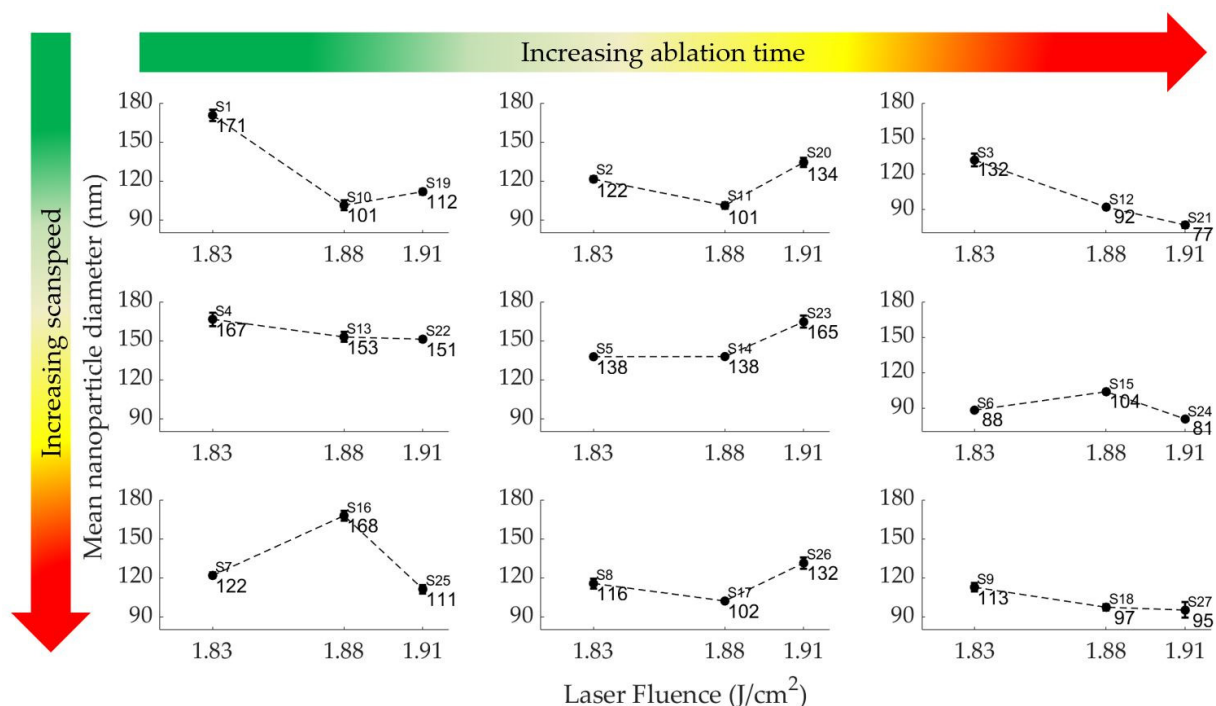
Figure 6. Effect of laser fluence on nanoparticle mean diameter (nm).
