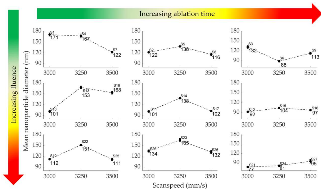
Figure 7. Effect of laser scan speed on nanoparticle mean diameter (nm).
