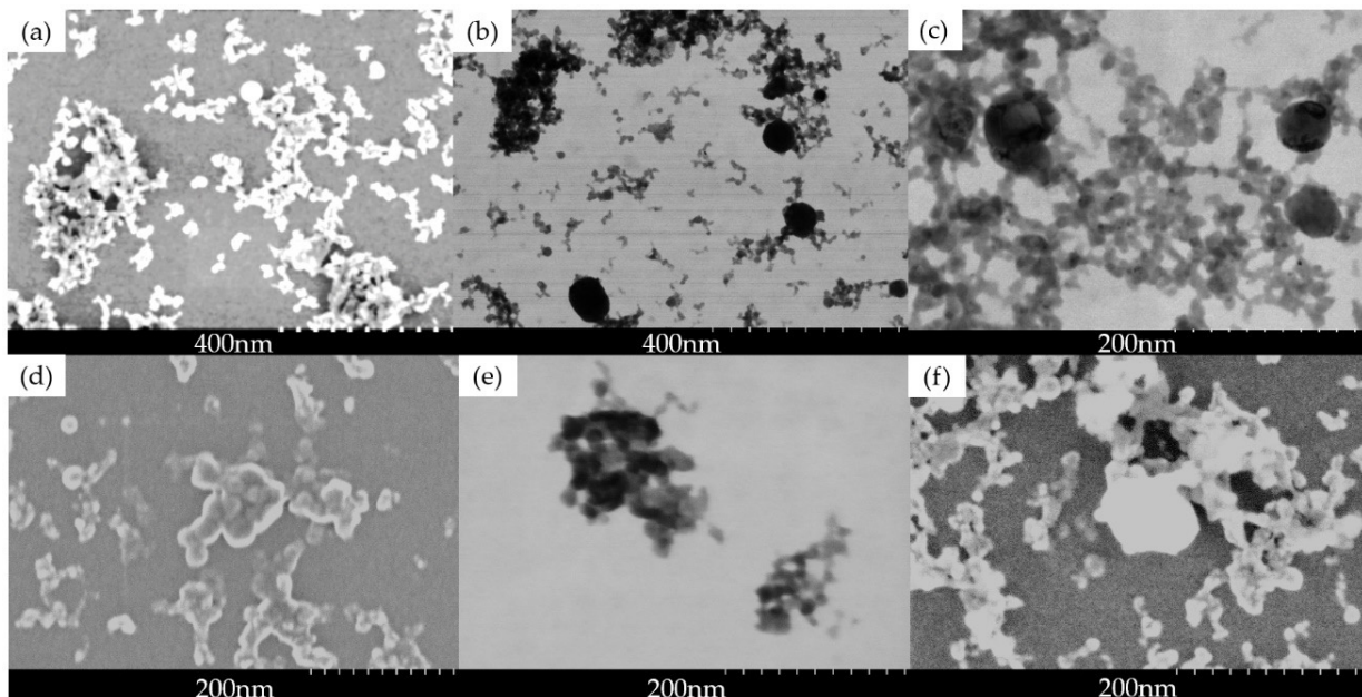
Figure 8. SEM images: (a) SEM image of sample 27C at 400 nm magnification and 30 kV acceleration voltage. (b) SEM image of sample 9C at 400 nm magnification and 20 kV acceleration voltage. (c) SEM image of sample 9C at 200 nm magnification and 30 kV acceleration voltage. (d) SEM image of sample 27C at 200 nm magnification and 30 kV acceleration voltage. (e) SEM image of sample 21C at 200 nm magnification and 20 kV acceleration voltage. (f) SEM image of sample 9C at 200 nm magnification and 9 kV acceleration voltage.
