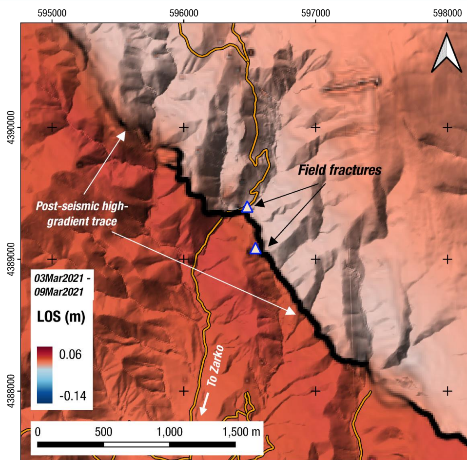
Fig. 17: Post-seismic interferogram (track 102, ascending orbit) showing alignment of phase gradient (thick black line) with location of surface cracks observed in the field (see Fig. 12d for a field photograph).
