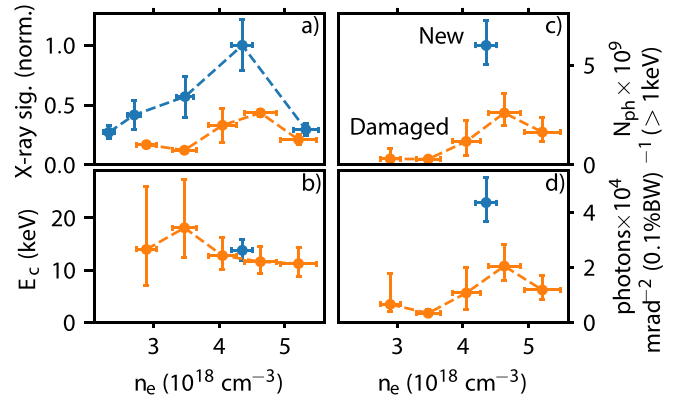
Figure 4. (a) Normalised total x-ray detector signal, (b) synchrotron spectrum critical energy, (c) number of photons per pulse above 1 keV and (d) peak spectral intensity per solid angle, all as functions of plasma density. The orange markers show results for a damaged gas cell (run 6 in figure 6) while the blue show results for a repaired cell (run 7 in figure 6) with a new exit aperture plate. Note, the critical energy and photon yield were only diagnosed at a single density for the newly repaired gas cell. Error bars include the measurement uncertainties and the standard error from averaging multiple shots.
