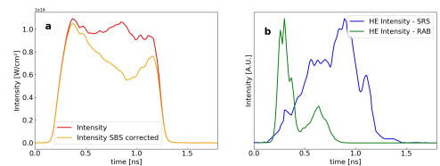
FIG. 16: (a) Experimental laser pulse shape (red) and SBS-corrected laser pulse shape (orange). (b) The intensity of HE beam is assumed to exactly follow either SRS reflected power measured by the SABS (blue) or RAB signal computed by CHIC (green).
