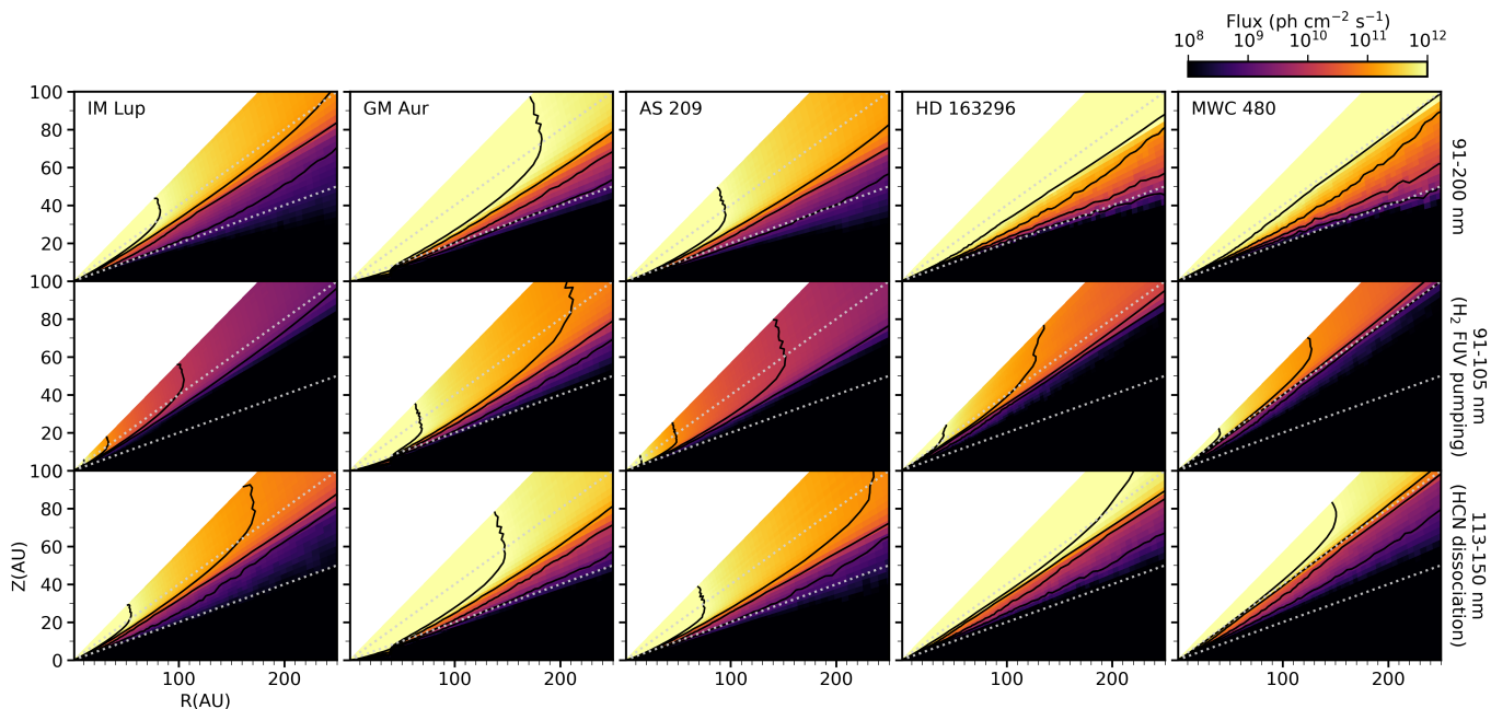
Figure 9. Toy disk modeling results showing the distribution of total UV flux (top row) as well as the flux within the wavelength bins 91-105 nm (i.e. CN formation via FUV pumping of \text{H}_2 ; middle row) and 113-150 nm (HCN selective photodissociation; bottom row). Contour levels correspond to 10^9 , 10^{10} , 10^{11} , and 10^{12} photon \text{cm}^{-2} \text{s}^{-1} . Dotted grey lines mark elevations with z/r=0.2 and 0.4 for reference.
