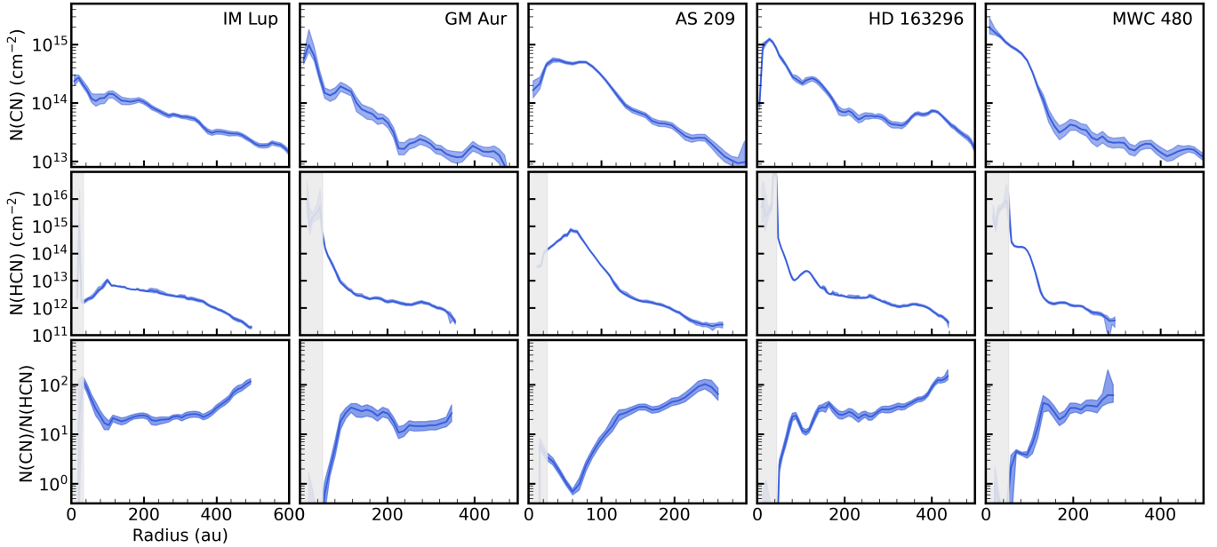
Figure 4. CN (top) and HCN (middle) column densities, and the CN/HCN column density ratios (bottom), derived from hyperfine fitting. Solid blue lines represent the median and shaded blue regions represent the 16th–84th percentiles of the MCMC posteriors. The greyed-out regions represent disk radii for which HCN line blending is too severe to allow reliable constraints on the column densities.
