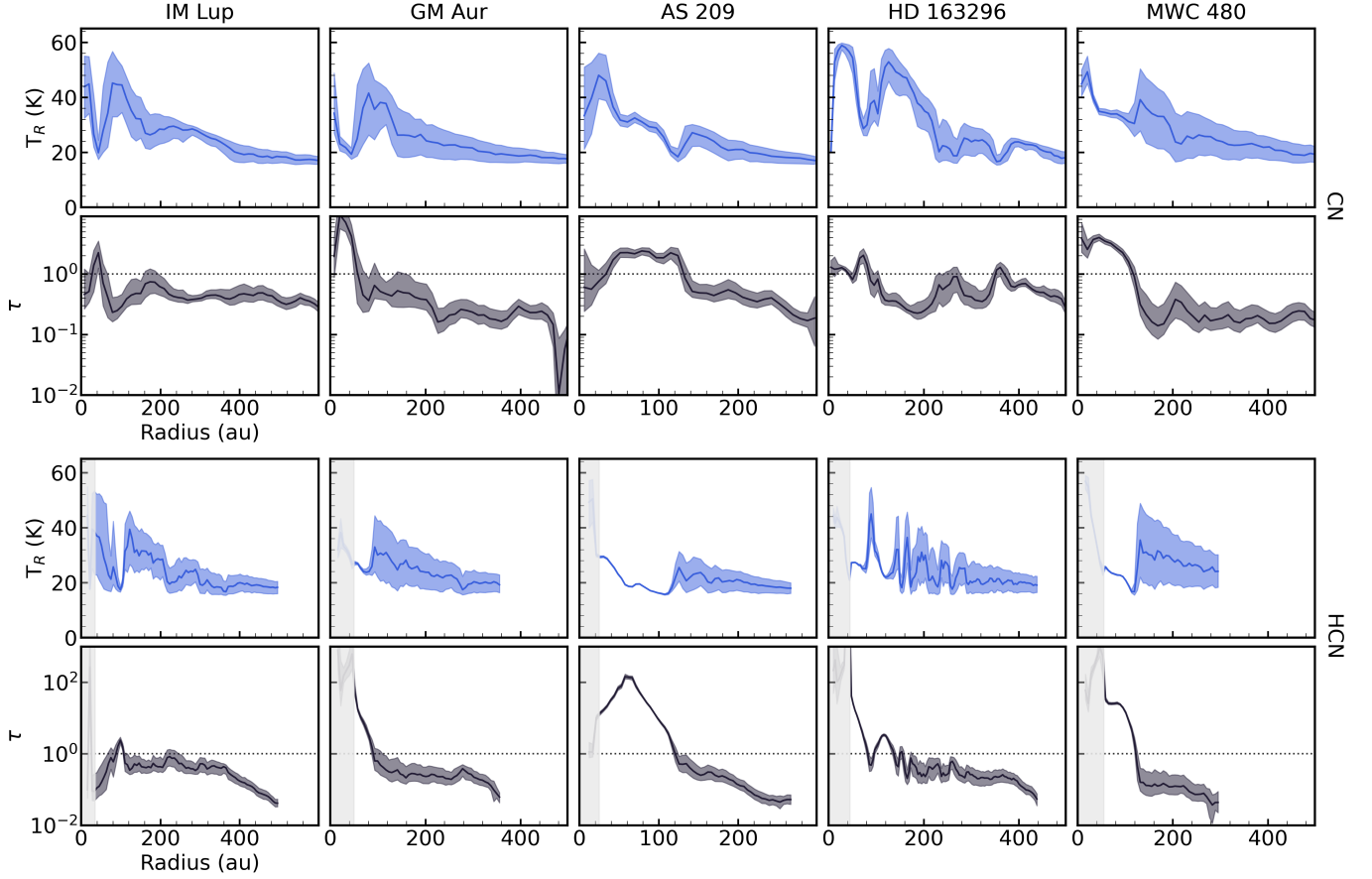
Figure 12. CN and HCN rotational temperature (blue) and optical depth (grey) profiles derived from hyperfine fitting. \tau is shown for the main hyperfine component (i.e. 113.491 GHz for CN and 265.8865 for HCN). Shaded regions represent the 16th-84th percentiles of the fit posteriors, and solid lines represent the median. \tau=1 is marked with dotted horizontal lines.
