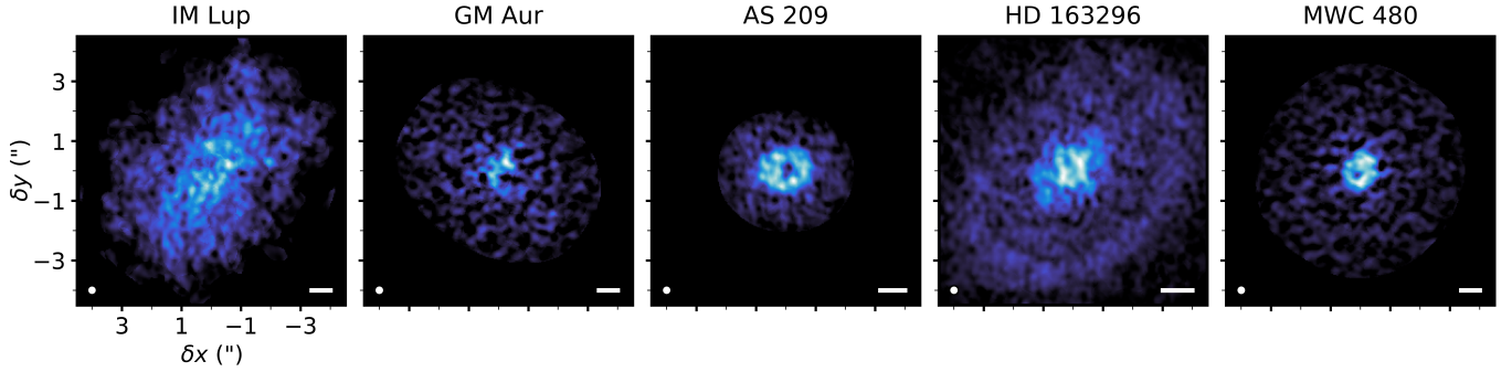
Figure 1. Presentational moment zero maps of CN N=1–0 emission (including the two hyperfine components at 113.488 and 113.491 GHz) towards the five MADS disks. To better illustrate weak emission features, integrated intensities are shown with a power-law color stretch. Color scales are normalized to each individual image. In each panel, the restoring beam is shown in the lower left and a 100 au scale bar is shown in the lower right.
