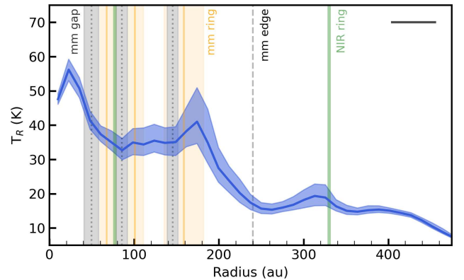
Figure 8. CN rotational temperature profile derived from joint fitting of N=1-0 and N=2-1 lines in HD 163296. Vertical lines represent the locations of millimeter rings (solid orange), millimeter gaps (dotted grey), the millimeter disk edge (dashed grey), and NIR rings (solid green). For millimeter features, the measured substructure widths are indicated with shaded regions. The restoring beam FWHM is shown with a horizontal black line.
