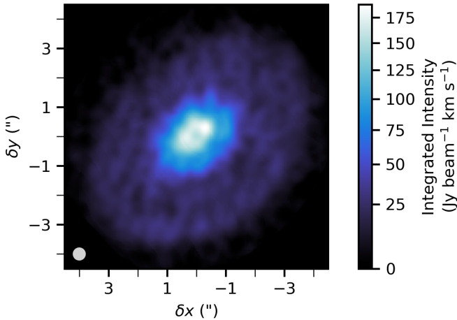
Figure 10. CN N=2-1 moment zero map in HD 163296. To better illustrate weak emission features, integrated intensities are shown with a power-law color stretch. The restoring beam is shown in the bottom left.
