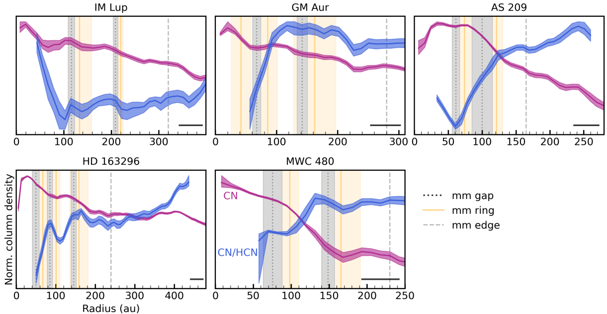
Figure 5. Normalized column density profiles of CN and CN/HCN (pink and blue lines, respectively) with millimeter dust features overplotted. Solid orange and dotted grey vertical lines represent the positions of millimeter rings and gaps, respectively. The substructure widths are indicated with shaded regions. The millimeter edge is shown as a dashed grey line. Substructure properties are taken from Law et al. (2021a). Horizontal black lines show the restoring beam FWHM of the line data.
