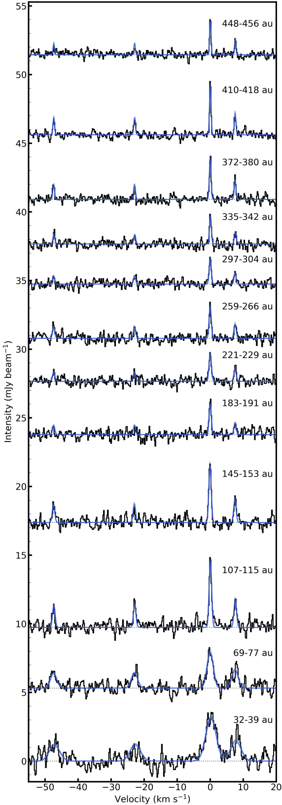
Figure 3. Example radial spectra of the CN N=1-0 hyperfine components in HD 163296 (black lines), averaged within a \pm 30^\circ wedge along the disk major axis. Draws from the spectral line fit posteriors are shown in blue. Spectra are offset for clarity, and the radial range of each spectrum is indicated on the right.
