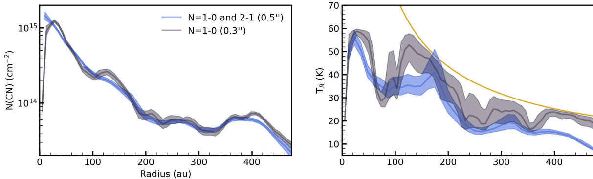
Figure 11. The column density and excitation temperature profiles in HD 163296 when the CN N=1–0 hyperfine components are fit alone (grey lines) compared to a joint fit of the N=1–0 and 2–1 lines (blue lines). The temperature profile derived from ^{12}\text{CO} in Law et al. (2021b) is shown as a gold line.
