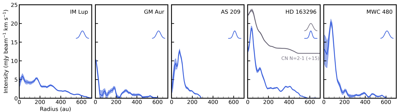
Figure 2. CN N=1–0 deprojected radial intensity profiles, including only pixels within a \pm 30^\circ wedge along the disk major axis. CN N=2–1 is also shown for HD 163296 (grey line), scaled down by a factor of 15 and offset for clarity. Shaded regions represent the uncertainties in each radial bin, as described in Law et al. (2021a). The synthesized beams are shown in the upper right of each panel.
