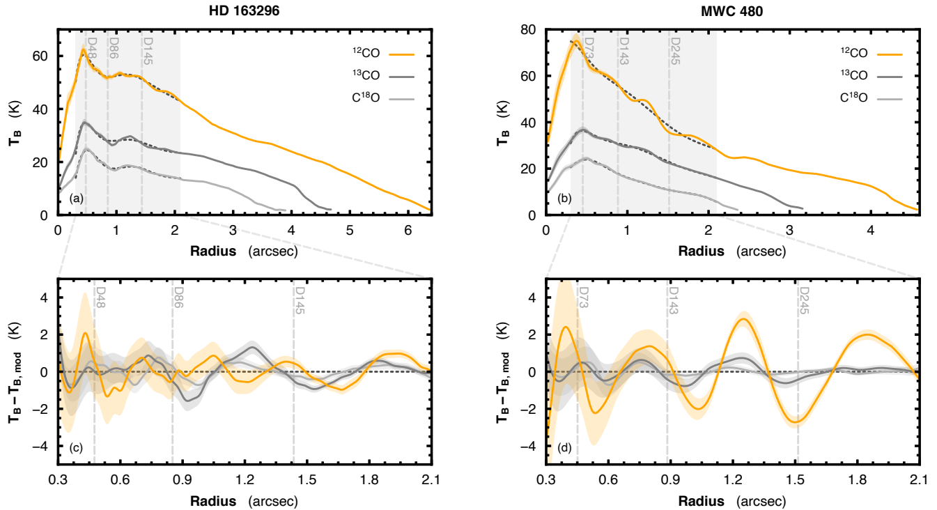
Figure 6. Azimuthally averaged T_B profiles for CO J = 2 - 1 isotopologue emission in HD 163296, panels (a) and (c), and MWC 480, (b) and (d). In all panels, the shaded regions show the 1\sigma uncertainty while the vertical dashed lines show the locations of gaps in the mm continuum. Panels (c) and (d) show a zoom-in of panels (a) and (b), respectively, after subtracting a smooth background model, T_{B,\text{mod}} , shown as a dotted black line in panels (a) and (b). The background model is a 10th-order polynomial fit to the profile between 0''.3 and 4'' for ^{12}\text{CO} and ^{13}\text{CO} , and between 0''.3 and 2'' for \text{C}^{18}\text{O} . The shaded regions in panels (a) and (b) show the extent of panels (c) and (d), respectively.
