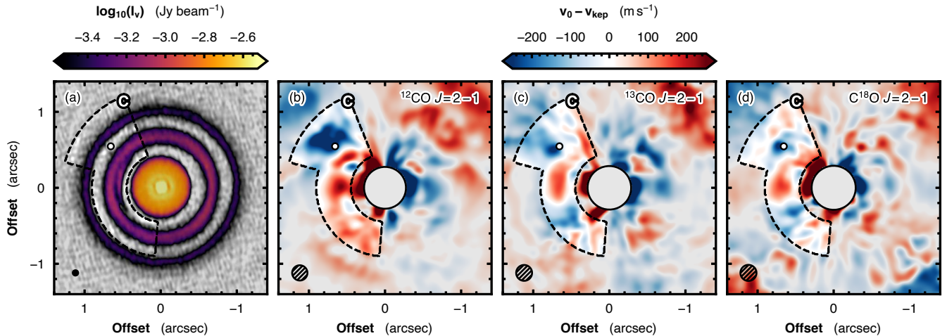
Figure 11. Kinematic structures around the continuum vortex and proposed KPS in the inner disk of HD 163296. Panel (a) shows the spatially deprojected 1.25 mm continuum data from DSHARP (Andrews et al. 2018; Isella et al. 2018) with the vortex and KPS region, box C in Fig. 2, outlined. Panels (b), (c) and (d) show similar zoom-ins of the v_0 residuals for ^{12}\text{CO} , ^{13}\text{CO} and \text{C}^{18}\text{O} , respectively. In all panels, the proposed planet location from Pinte et al. (2020) is plotted. All v_0 residual maps share the same color scaling. A representative beam size is shown in the bottom left of each panel, taking into account the deprojection.
