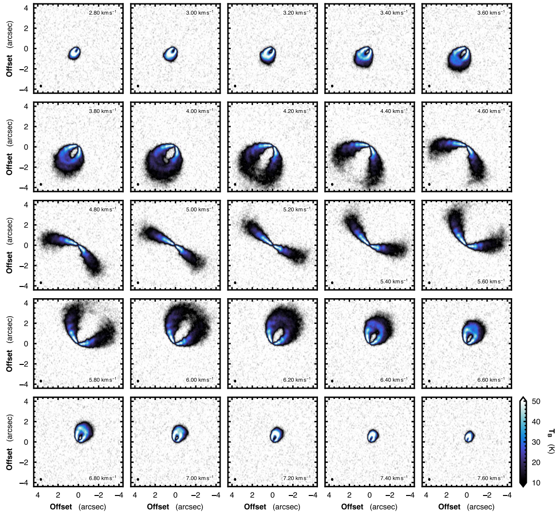
Figure 19. Channel maps of ^{12}\text{CO } J = 2 - 1 emission in MWC 480. The color scaling has been chosen to highlight the morphology of the emission from the line wings. The velocity is given for each channel, as well as the synthesized beam shown in the bottom left of each panel.
