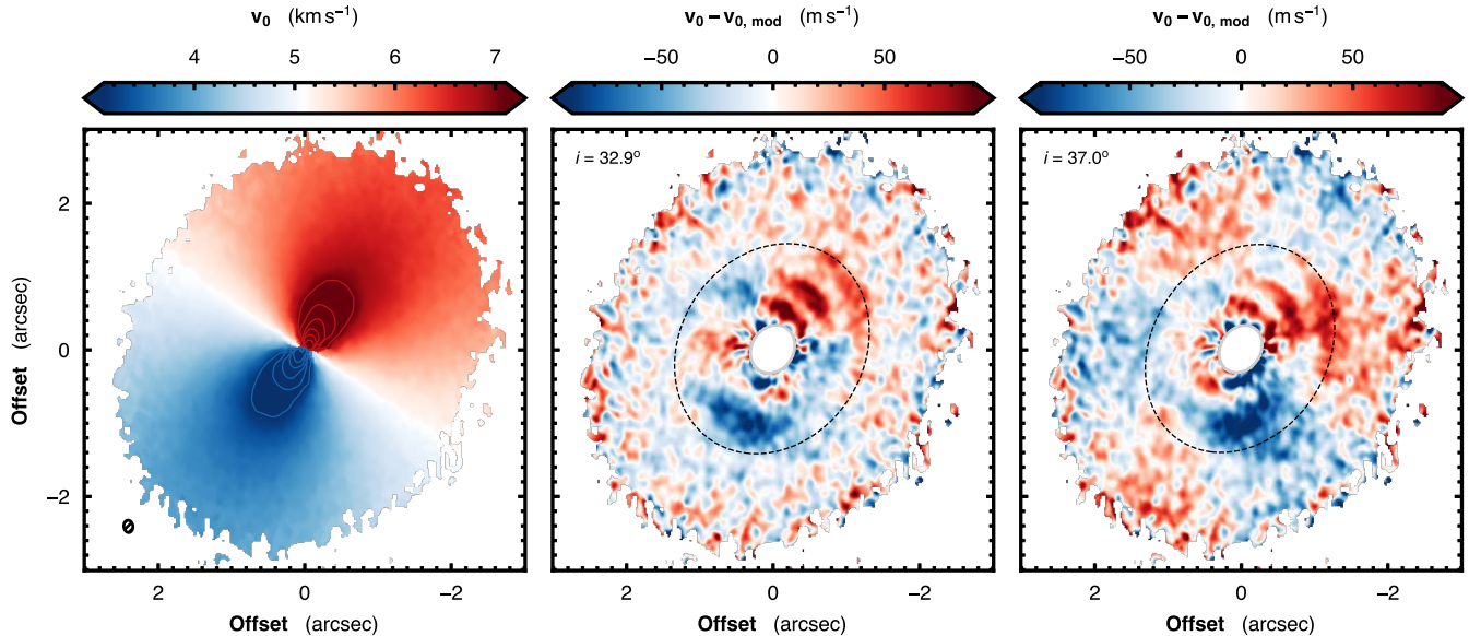
Figure 15. Left: The v_0 map of ^{13}\text{CO} (2-1) in MWC 480. The synthesized beam is shown by the ellipse in the lower left corner of the panel. Center: Residuals from a Keplerian model where the inclination was allowed to vary. The fit only considered emission outside a (projected) radius of 1''.8 , shown by the dashed black line. Right: Residuals from a Keplerian model where the inclination was fixed to 37^\circ .
