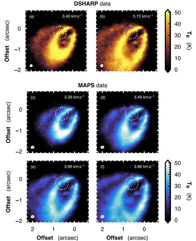
Figure 10. Channel maps of ^{12}\text{CO} J = 2-1 emission from the disk around HD 163296, centered on the proposed kinematic planetary signature reported by Pinte et al. (2020). The top two panels, (a) and (b) used DSHARP data (Andrews et al. 2018; Isella et al. 2018), while the bottom four panels, (c) through (f), use MAPS data. No clear “kink” is visible at the spatial resolution of the MAPS data. The dotted circle shows the region of interest.
