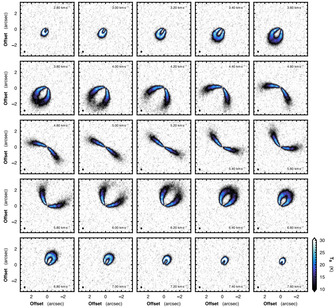
Figure 20. As Fig. 19 but for ^{13}\text{CO } J = 2 - 1 emission.
