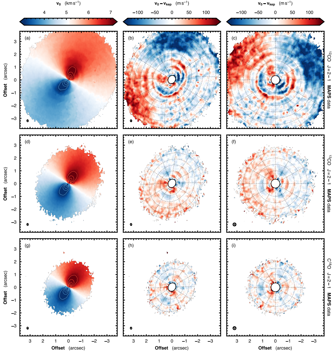
Figure 3. As Fig. 1, but for MWC 480. As this disk was not targeted by the DSHARP survey, only the MAPS data are shown. The disk rotates in an anti-clockwise direction in all frames. The beam size is shown in the bottom left of each panel. For the deprojected maps in the right hand column, the beam size is only representative as the deprojection results in a non-uniform spatial resolution across the image.
