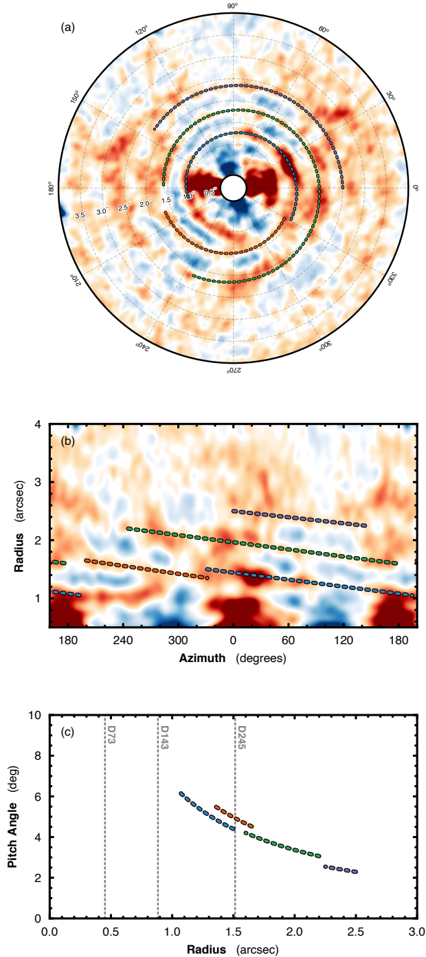
Figure 9. Panel (a) shows an annotated version of Fig. 8c, highlighting the spirals, show with colored dotted lines. Panel (b) is a polar deprojection of panel (a) to better demonstrate the spiral structure. The pitch angles for the spirals are shown in panel (c), with the locations of the continuum gaps annotated.
