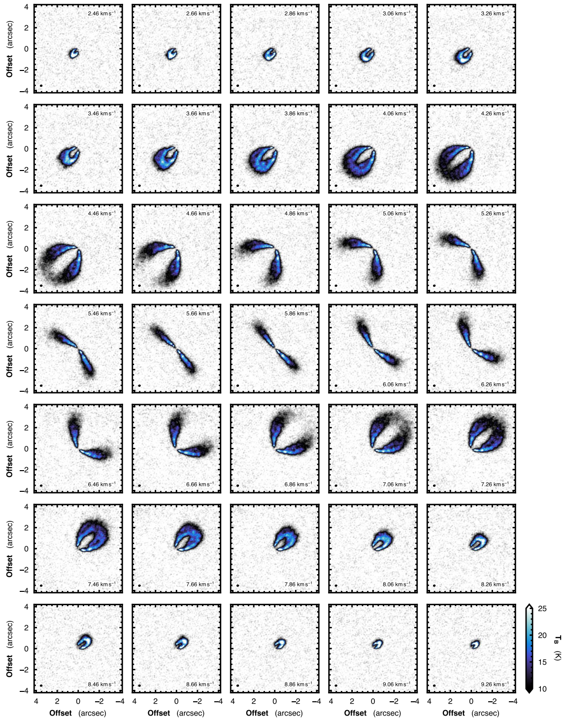
Figure 17. As Fig. 16, but for ^{13}\text{CO } J = 2 - 1 emission.
