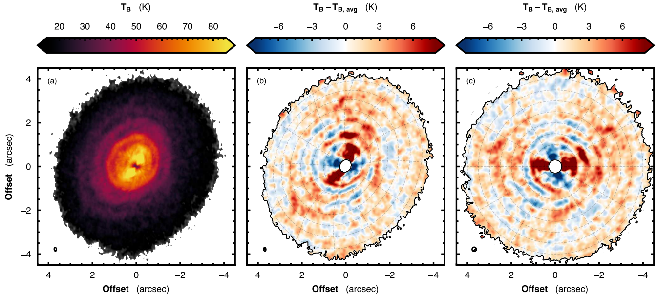
Figure 8. As Fig. 7 but for ^{12}\text{CO} in the disk of MWC 480. In all frames, the disk rotation is in an anti-clockwise direction.
