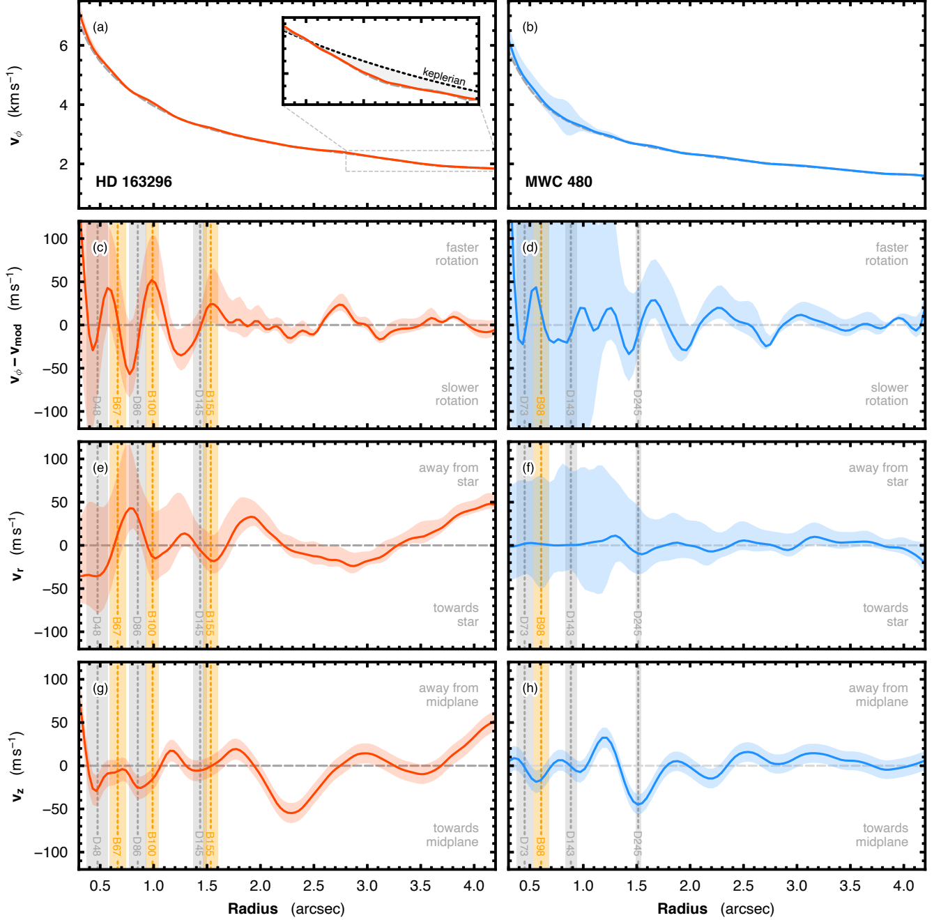
Figure 5. Azimuthally averaged radial profiles of the gas velocities in HD 163296, left, and MWC 480, right, traced by ^{12}\text{CO} . Panels (a) and (b) show v_\phi , while panels (c) and (d) show the residual of v_\phi after subtracting a baseline v_{\text{mod}} . The radial and vertical velocities are shown in panels (e) and (g) and (f) and (h) for HD 163296 and MWC 480, respectively. All velocities have been corrected for the inclination of the disk. Following Teague et al. (2019a), the baseline model, v_{\text{mod}} , used to highlight localized deviation in v_\phi is a 10th order polynomial fit to v_\phi . In (a), an inset highlights the difference between a purely Keplerian rotation profile, black dotted line, and the observed rotation profile and 10th order polynomial fit, gray dashed line, used for panel (c). The shaded regions show the 1\sigma uncertainties. Locations of the gaps and rings in the continuum are annotated in the lower three rows as vertical dashed lines with the gray and orange shading showing their width (Huang et al. 2018a). Note that the sign convention for radial velocity has been inverted relative to Teague et al. (2019b) such that positive v_r represent gas moving away from the star.
