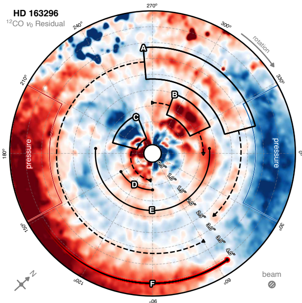
Figure 2. A zoom-in of Fig. 1c. A representative beam size is shown in the lower right, however due to the elevated emission surface, the true angular resolution varies across the map. The figure extends out to 4''.4 , and the color scaling ranges between residuals of \pm 180 \text{ m s}^{-1} . Residuals due to the pressure gradient slowing the rotation of the disk are observed along the major axis, marked as “pressure”. Three regions of large velocity deviations are marked by black boxes, centered at (r, \phi) = (2''.85, 305^\circ) , A, (1''.65, 315^\circ) , B, and (0''.9, 220^\circ) , C, all of which have extended structure shown by the dashed lines. The outer feature, A, is associated with the planet identified by Pinte et al. (2018a), while the in two, B and C, are likely associated with the potential “kink” reported by Pinte et al. (2020), or due to the asymmetry in the continuum emission (Isella et al. 2018). Two arc-like structures are also seen at radii of 1''.15 (116 au), and 1''.8 (182 au), shown by the solid lines, labeled D and E, respectively, in addition to a larger arc feature at 4''.1 (414 au), shown by the thick solid line with a faded end, annotated as F. It is unclear where this outer-most arc ends as the perturbation extends into a region dominated by pressure-modulated deviations.
