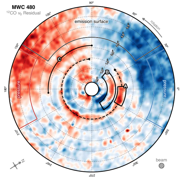
Figure 4. Annotated version of Fig. 3c, showing the features observed in the residual rotation map from ^{12}\text{CO} in the disk of MWC 480. The disk rotates in an anti-clockwise fashion. Residuals due to the pressure gradient slowing the rotation of the disk are observed along the major axis, marked as “pressure”, with similar systematic features likely due to a misspecified emission surface marked as “emission surface”. The most prominent is an arc extending almost the full azimuth of the disk at 1''.5 with a peak marked by a solid annulus, labeled A, with an inner arc at 0''.95 , labeled B. An additional tentative arc is annotated as arc C at 2''.1 . A representative beam size is shown in the lower right, however due to the elevated emission surface, the true beam size varies across the map.
