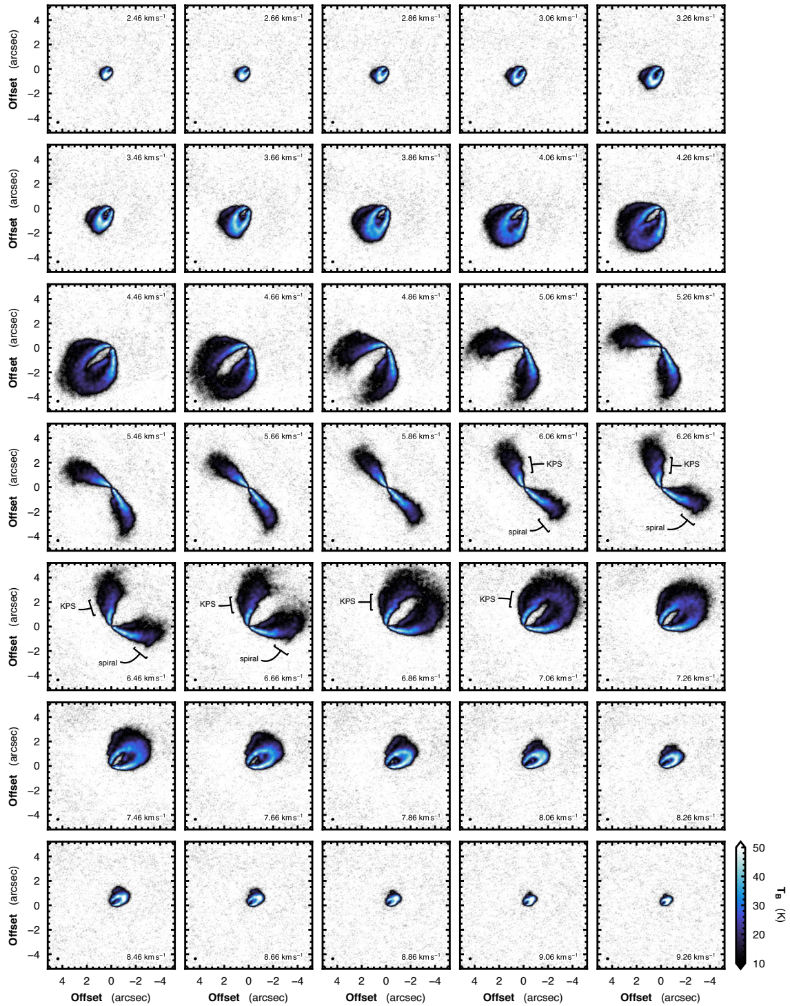
Figure 16. Channel maps of ^{12}\text{CO } J = 2 - 1 emission in HD 163296. The color scaling has been chosen to highlight the morphology of the emission from the line wings. The velocity is given for each channel, as well as the synthesized beam shown in the bottom left of each panel. Regions where the KPS and spiral are most visible are annotated.
