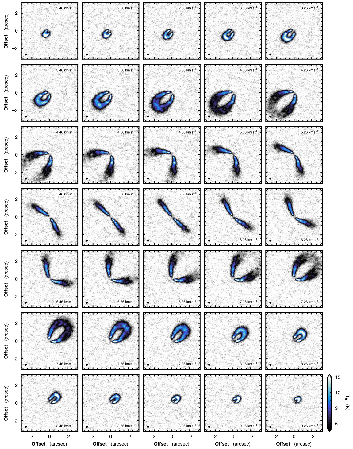
Figure 18. As Fig. 16, but for C^{18}O J=2-1 emission.
