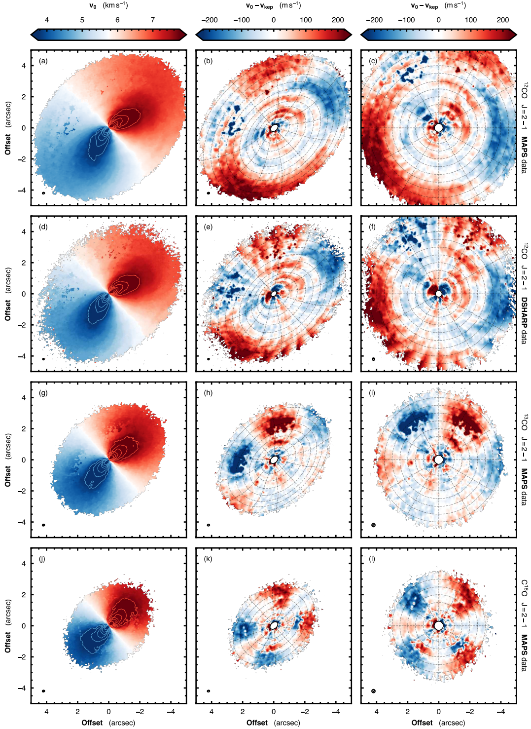
Figure 1. Gallery of v_0 maps for different J = 2 - 1 CO isotopologue emission from the disk around HD 163296 using both MAPS and DSHARP data (Andrews et al. 2018; Isella et al. 2018). The left column shows the raw v_0 map, the central column shows the residuals after subtracting a best-fit Keplerian rotation model, and the right column shows the residuals deprojected into a face-on orientation accounting for the elevated emission surface. Solid colored contours in the left panel show iso-velocity contours of v_{\text{LSR}} \pm \{2, 2.5, 3, \dots\} km s ^{-1} . Dashed black contours in the central and right hand columns show contours of constant radius and azimuth in the disk frame, with intervals of 0.5 and 30°, respectively. The beam size is shown in the bottom left of each panel. For the deprojected maps in the right hand column, the beam size is only representative as the deprojection results in a non-uniform spatial resolution across the image. The disk rotates clockwise in all panels.
