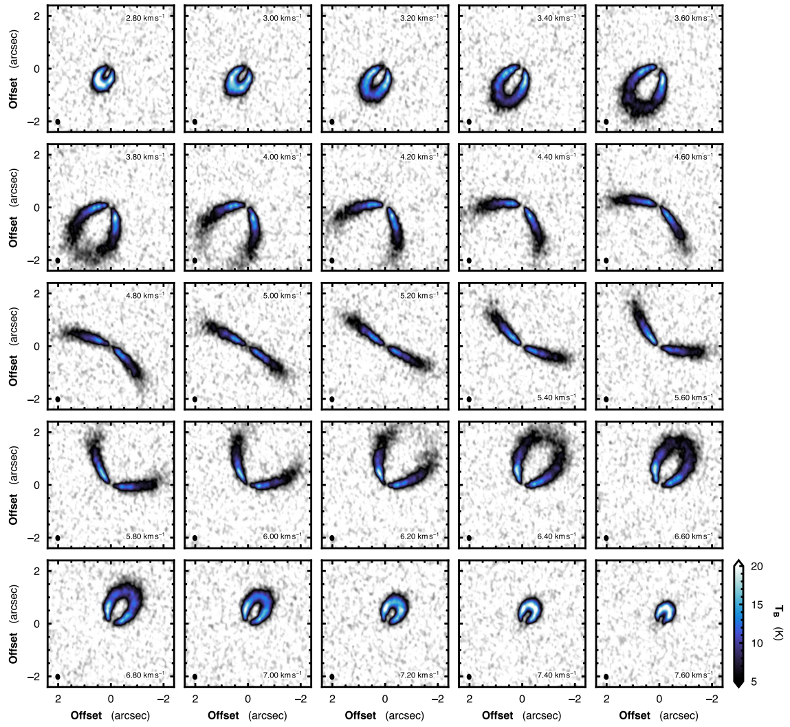
Figure 21. As Fig. 19 but for \text{C}^{18}\text{O } J=2-1 emission.
