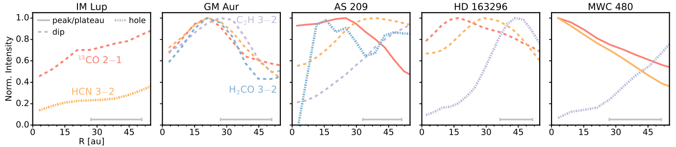
Figure 24. Normalized radial intensity profiles of select lines covered in Band 6 at 0''.15 in the inner 50 au. Species are color-coded, as in Figures 15, 16, 17, 22. Classifications, as in Figure 23, of central peaks/plateaus, dips, and holes are shown as solid, dashed, and dotted lines, respectively. The FWHM of the synthesized beam is shown by a horizontal bar in the lower right corner of each panel.
