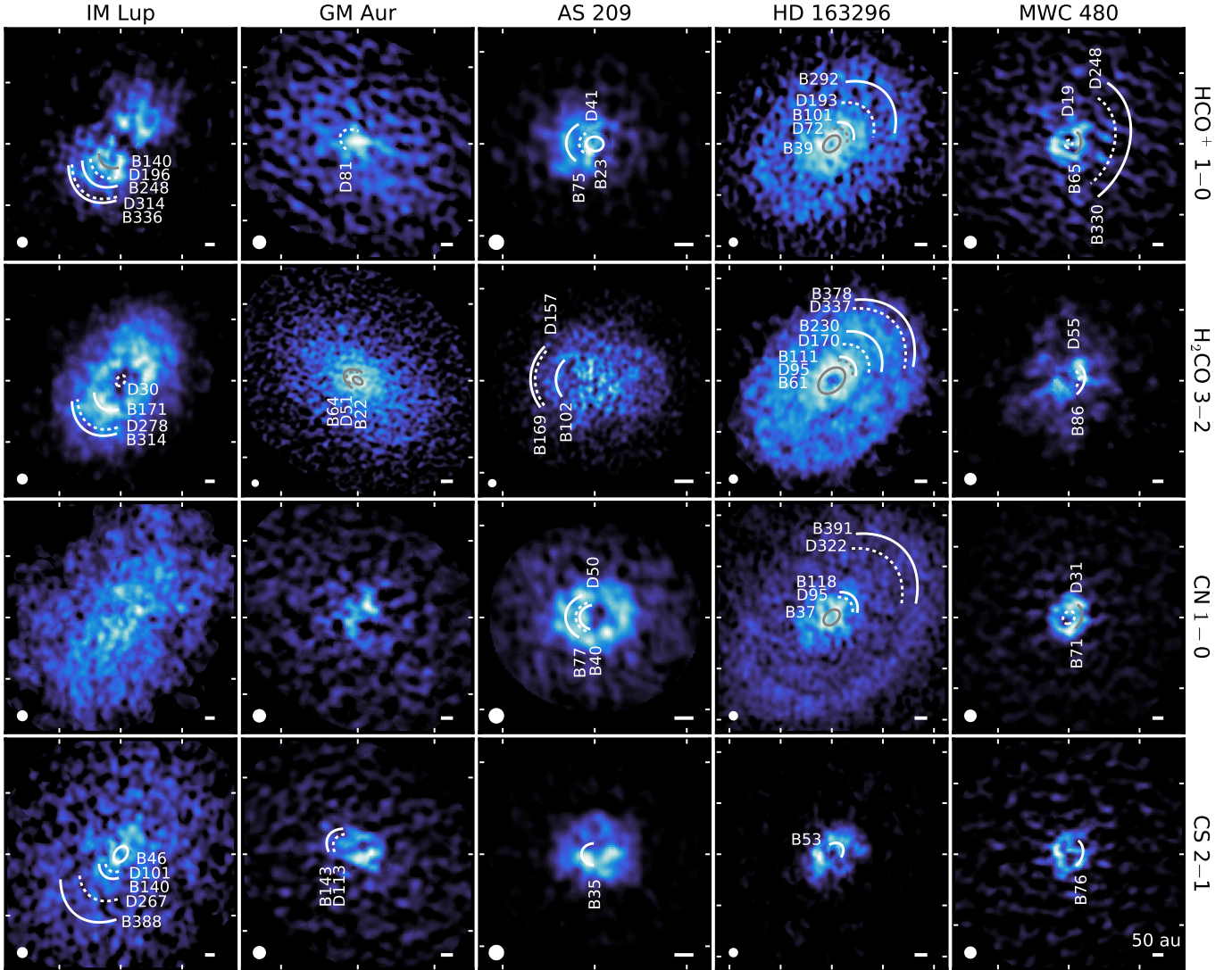
Figure 5. Zeroth moment maps of \text{HCO}^+ , \text{H}_2\text{CO} , \text{CN} , and \text{CS} lines for the MAPS sample, ordered from left to right by increasing stellar mass (see Table 1 in Oberg et al. (2021)). Axes are angular offsets from the disk center with each white tick mark represents a spacing of 2'' . Color stretches were individually optimized and applied to each panel to increase the visibility of substructures. Care should thus be taken when comparing between panels, and instead, we recommend using the corresponding radial profiles in Figure 11 for this purpose. Chemical substructures from Table 3 in the form of rings and gaps are marked by solid and dotted arcs, respectively, with azimuthal extents and colors chosen for maximal visual clarity. The synthesized beam and a scale bar indicating 50 au is shown in the lower left and right corner, respectively, of each panel.
