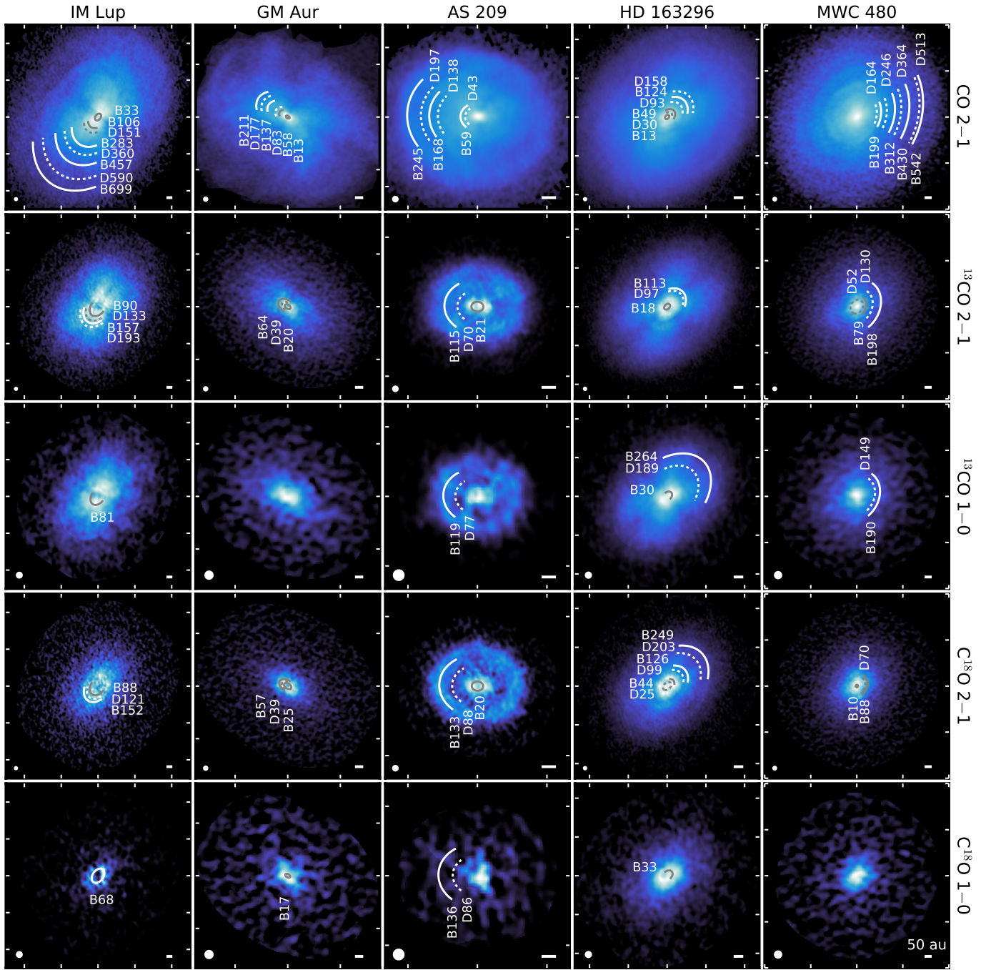
Figure 3. Zeroth moment maps of CO, ^{13}\text{CO} , and \text{C}^{18}\text{O} lines for the MAPS sample, ordered from left to right by increasing stellar mass (see Table 1 in Oberg et al. (2021)). Axes are angular offsets from the disk center with each white tick mark represents a spacing of 2'' . Color stretches were individually optimized and applied to each panel to increase the visibility of substructures. Care should thus be taken when comparing between panels, and instead, we recommend using the corresponding radial profiles in Figure 9 for this purpose. Chemical substructures from Table 3 in the form of rings and gaps are marked by solid and dotted arcs, respectively, with azimuthal extents and colors chosen for maximal visual clarity. Several inner low-contrast CO 2-1 substructures in IM Lup (D50, B68, D80) and HD 163296 (D71, B81) are omitted for visual clarity. The synthesized beam and a scale bar indicating 50 au is shown in the lower left and right corner, respectively, of each panel.
