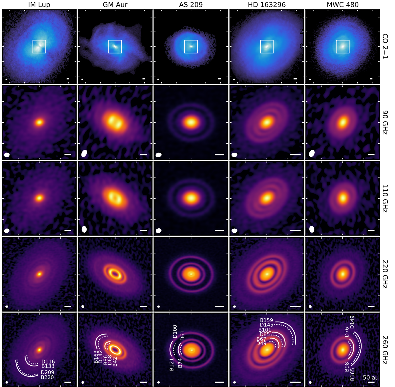
Figure 1. Zeroth moment maps of CO 2–1 and continuum images for the MAPS sample, ordered from left to right by increasing stellar mass (see Table 1 in Oberg et al. (2021)). Axes are angular offsets from the disk center and the white rectangle overlaid on the CO 2–1 zeroth moment maps defines the field of view of the continuum images. Each tick mark is 2'' and 1'' for the CO 2–1 and continuum images, respectively. Color stretches were individually optimized and applied to each panel to increase the visibility of substructures. Care should thus be taken when comparing between panels, and instead, we recommend using the corresponding radial profiles in Figure 14 for this purpose. Continuum substructures, as described in Section 3.4, are labeled on the 260 GHz continuum images following the nomenclature of Huang et al. (2018b). Rings and gaps are shown as solid and dotted arcs, respectively, with azimuthal extents chosen for maximal visual clarity. The synthesized beam and a scale bar indicating 50 au is shown in the lower left and right corner, respectively, of each panel.
