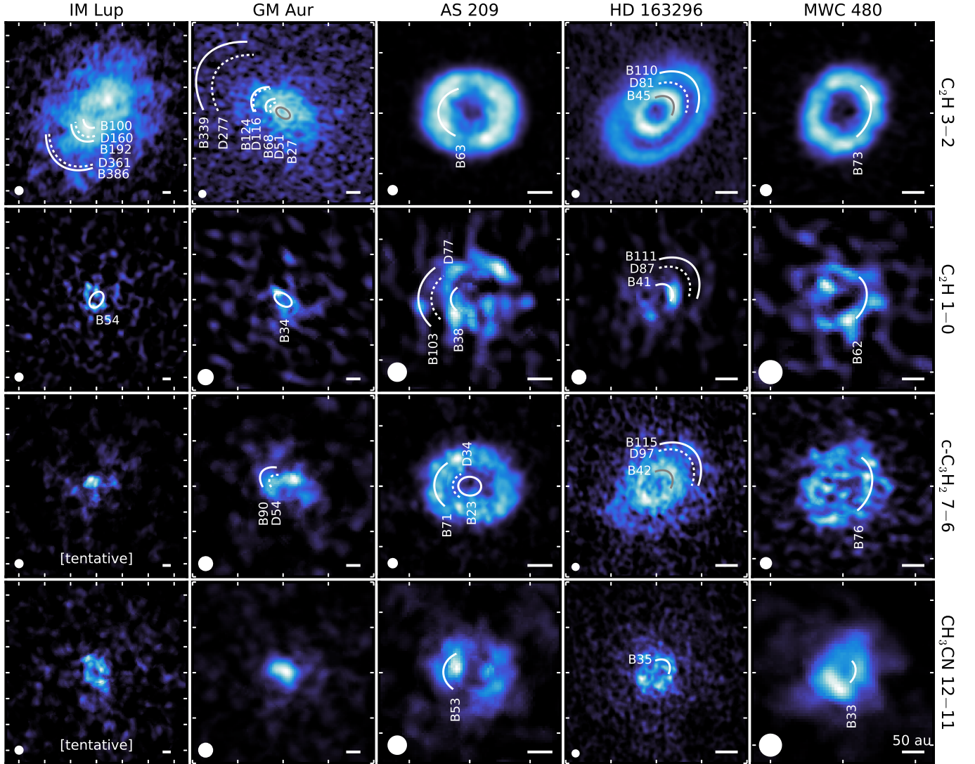
Figure 4. Zeroth moment maps of C_2H , c-C_3H_2 , CH_3CN lines for the MAPS sample, ordered from left to right by increasing stellar mass (see Table 1 in Oberg et al. (2021)). Axes are angular offsets from the disk center with each white tick mark represents a spacing of 1'' . Color stretches were individually optimized and applied to each panel to increase the visibility of substructures. Care should thus be taken when comparing between panels, and instead, we recommend using the corresponding radial profiles in Figure 10 for this purpose. Chemical substructures from Table 3 in the form of rings and gaps are marked by solid and dotted arcs, respectively, with azimuthal extents and colors chosen for maximal visual clarity. The synthesized beam and a scale bar indicating 50 au is shown in the lower left and right corner, respectively, of each panel.
