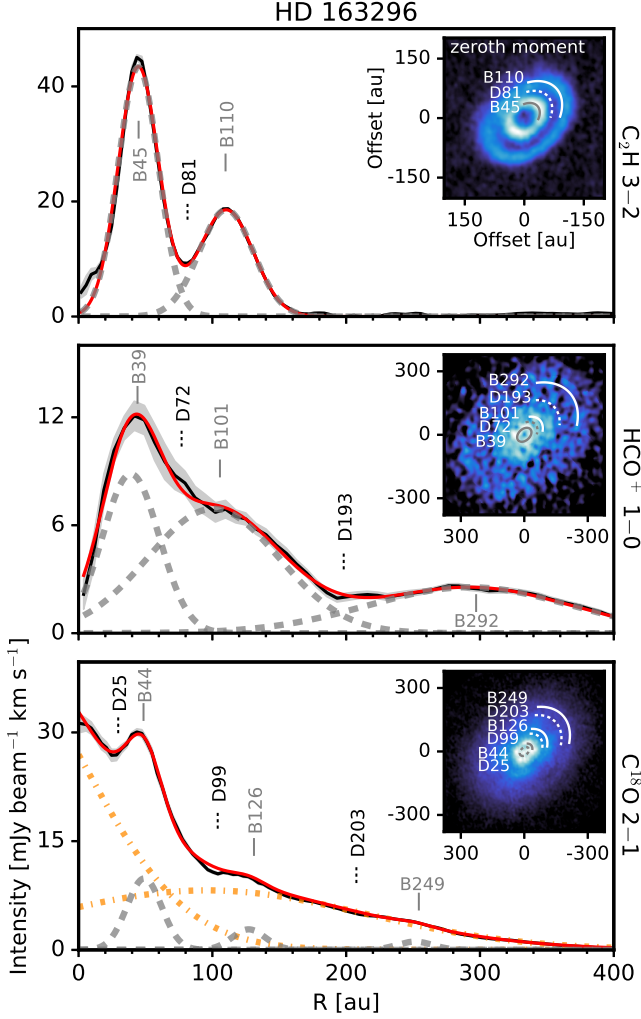
Figure 8. Example Gaussian decomposition for \text{C}_2\text{H} 3–2 (top), \text{HCO}^+ 1–0 (middle), and \text{C}^{18}\text{O} 2–1 (bottom) in HD 163296. The red solid line indicates the composite fit, while individual Gaussian profiles are shown as dashed gray lines. The orange dash-dotted lines in the bottom panel are Gaussians used to remove the broad and smoothly decreasing background in \text{C}^{18}\text{O} 2–1. The intensities of the low-amplitude Gaussians at \sim 130 and 250 au have each been multiplied by a factor of 3 for visual clarity. The insets show zeroth moment maps with axes labeled as offsets in au from the disk center. Chemical substructures are marked by solid and dotted arcs, indicating bright and dark features, respectively.
