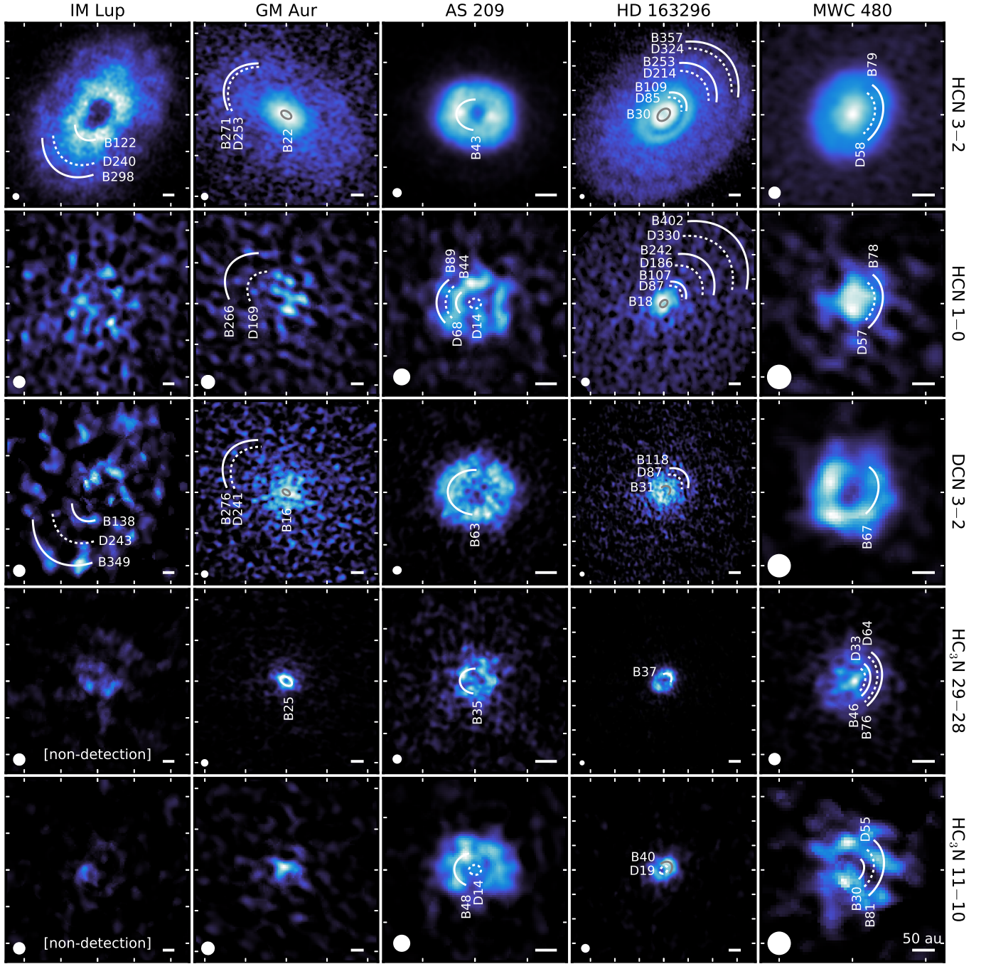
Figure 6. Zeroth moment maps of HCN, DCN, and \text{HC}_3\text{N} lines for the MAPS sample, ordered from left to right by increasing stellar mass (see Table 1 in Oberg et al. (2021)). Axes are angular offsets from the disk center with each white tick mark represents a spacing of 1'' . Color stretches were individually optimized and applied to each panel to increase the visibility of substructures. Care should thus be taken when comparing between panels, and instead, we recommend using the corresponding radial profiles in Figure 12 for this purpose. Chemical substructures from Table 3 in the form of rings and gaps are marked by solid and dotted arcs, respectively, with azimuthal extents and colors chosen for maximal visual clarity. The synthesized beam and a scale bar indicating 50 au is shown in the lower left and right corner, respectively, of each panel.
