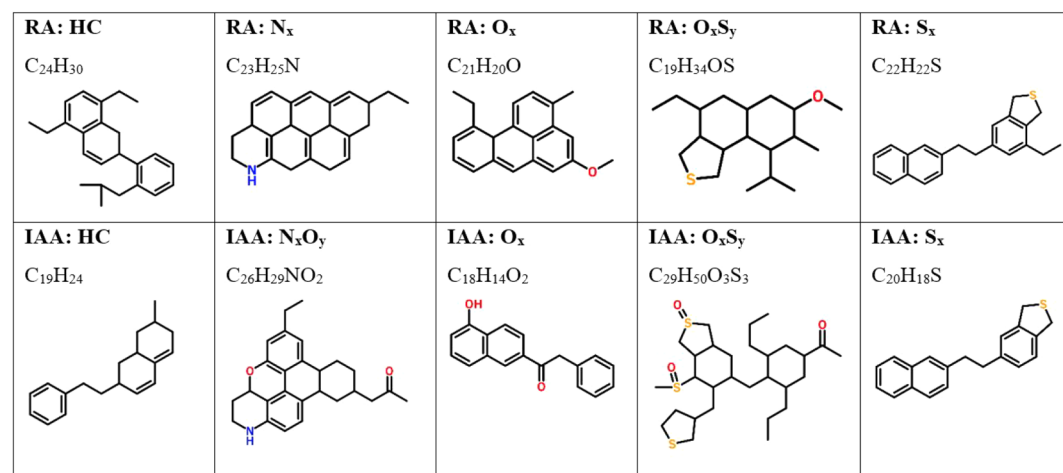
Figure 7. Proposed structures of RA (above) and IAA (below) fractions. These structures were optimized on the basis of the data given in Table 2.
