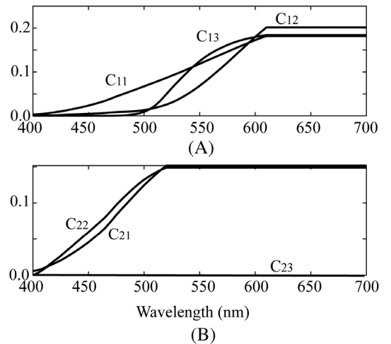
FIGURE 4 Spectral functions C_{i1}(\lambda) , C_{i2}(\lambda) , and C_{i3}(\lambda) for the fluorescent objects in Figure 1, where (A) represents the red fluorescent object ( i = 1 ) and (B) represents the yellow fluorescent object ( i = 2 )
