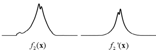
FIGURE 11 Comparison of the profiles of shading terms f_2(\mathbf{x}) and f_2'(\mathbf{x}) for the interreflection in Figures 9 and 10
