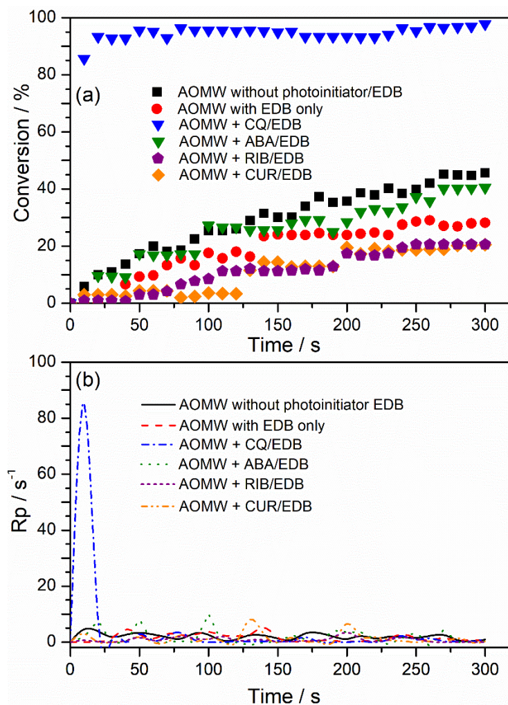
Figure 5. Monomer conversion (MC) curves obtained for synthesized polymers under blue light (a) and rates of polymerization (b).
