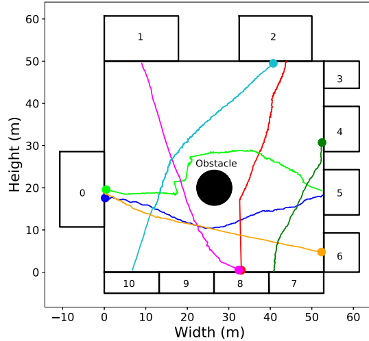
Figure 4: An outline of model environment over the Grand Central Station atrium in New York, including the central information kiosk obstacle. The solid lines represent trajectories of seven real pedestrians inferred from a video recorded at GCT. The circles mark the beginning of each pedestrian trajectory.
