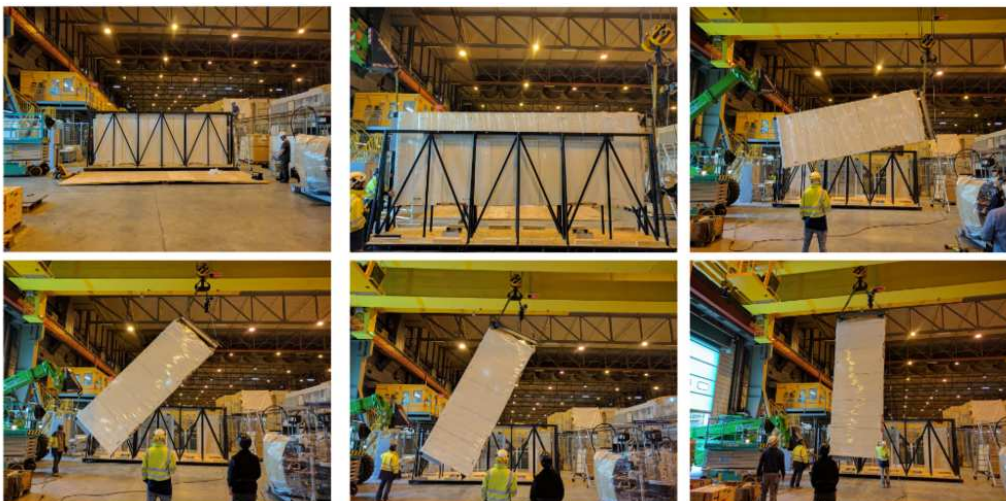
Figure 70. Arrival of an APA in EHN1 and its positioning. The upper left image shows the orientation of the APA as delivered, the lower right shows its vertical orientation when it is lowered into the material sas.
