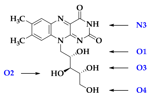
Scheme 1. Schematic diagram of the structure of riboflavin (RF). Typical labelling conventions have been applied to illustrate the possible deprotonation sites of a mono-anion deprotonomer (i.e., [\text{RF} - \text{H}]^- ).
