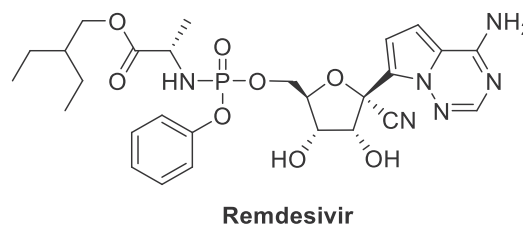
Fig. 2. Structure of remdesivir.
