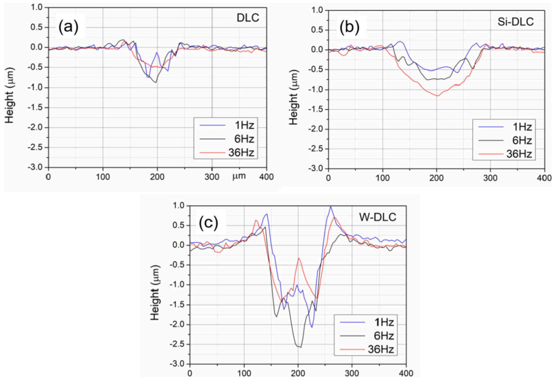
Fig. 11. Line profiles of the topography of the wear tracks on the DLC coatings after the sliding wear tests (total distance of 43.2 m) at reciprocating frequencies 1 Hz, 6 Hz and 36 Hz: (a) DLC, (b) Si-DLC, and (c) W-DLC.
