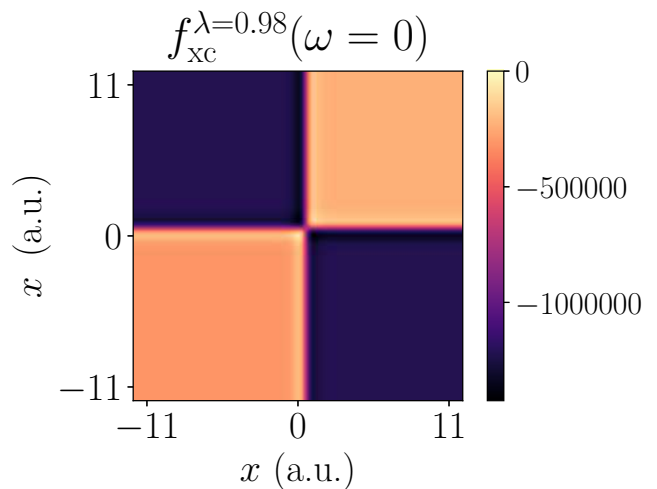
FIG. 7. The exact f_{\text{xc}}^{\lambda}(x, x', \omega = 0) for the double well system at \lambda = 0.98 , i.e. at a discrete value of \lambda that is sampled along the adiabatic connection.
