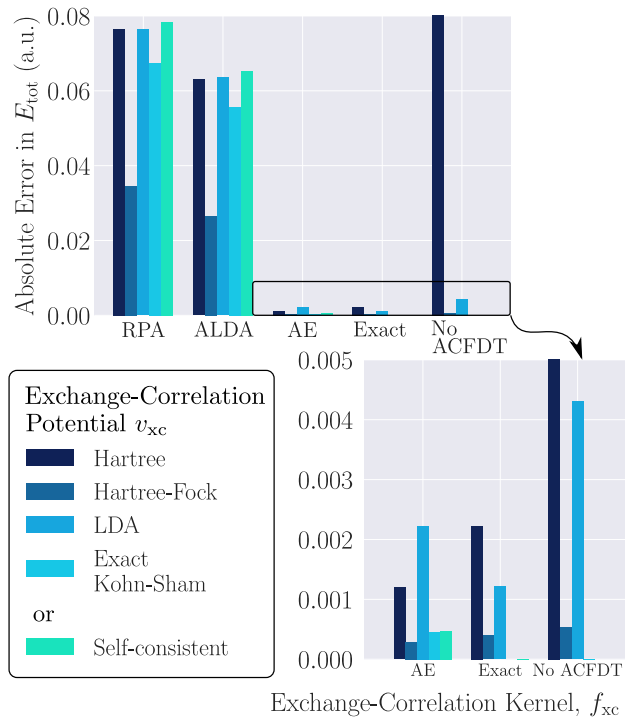
FIG. 3. Absolute error in the infinite potential well total energy across a variety of approximate ACFDT total energies, see caption of Figure 3 in the main text.
