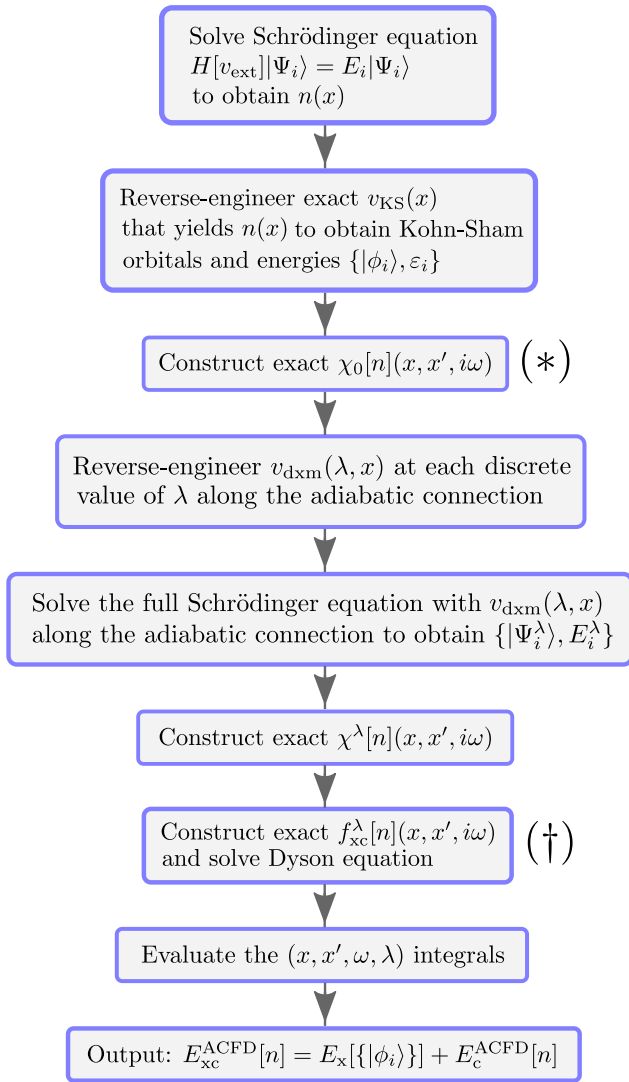
FIG. 1. A flow chart depicting the course of action taken to evaluate the exact ACFDT total energy E_c^{\text{ACFD}}[n] at the exact interacting ground-state density n . This procedure is modified in order to investigate approximate ACFDT approaches as follows: (*) a non-interacting Kohn-Sham calculation is performed with some approximate v_{\text{xc}}[n] , and then the algorithm proceeds with the corresponding approximate non-interacting response function, (†) rather than calculate and utilize the exact f_{\text{xc}}^\lambda[n] , an approximate functional f_{\text{xc}}^\lambda[n] is chosen and used alongside \chi_0[n] to solve the Dyson equation Eq. (10), ultimately yielding an approximate many-body response function \chi^\lambda[n] .
