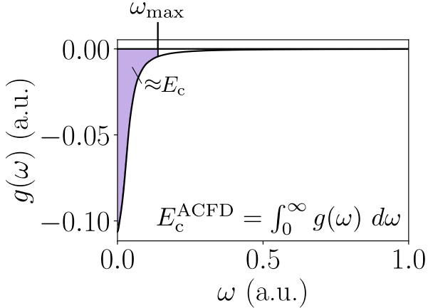
FIG. 10. The exact \omega -dependent integrand g(\omega) of the ACFDT correlation energy expression is depicted for the slab system. Analytic integration allows us to terminate the integration at some finite \omega_{\max} in order to determine the amount of correlation energy contained in the curve at frequencies \omega \leq \omega_{\max} .
