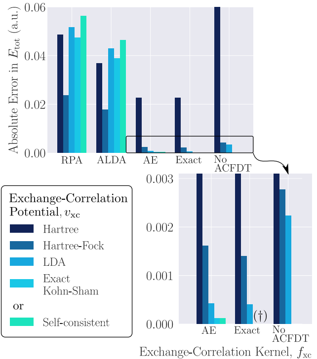
FIG. 3. Absolute error in the atomic total energy across a variety of approximate ACFDT total energies. Each of the first four groups of colored bars is labeled with the approximate f_{xc}[n] used to specify E^{ACFDT}[n] , while the fifth group (‘No ACFDT’) denotes a conventional ground-state Kohn-Sham calculation, for comparison. The first four bars of each group indicate the approximate v_{xc}[n] used to generate the density (and orbitals) at which E^{ACFDT}[n] is evaluated, while the fifth bar (cyan) indicates that the input density was determined self-consistently (i.e. it minimizes the applicable ACFDT total energy functional). The lower bar chart enlarges the outlined region in the upper bar chart. (†) At this position, there are two bars of zero height, i.e. the exact interacting ground-state density coincides with the density that minimizes the energy functional, both of which return the exact ground-state energy.
