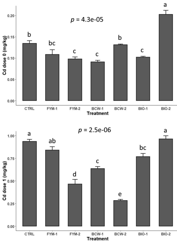
Fig. 1 Concentrations of the bioavailable fractions of Cd in soil contaminated by HMs at dose 0 (a), dose 1 (b) and dose 2 (c) after treatment by different organic materials. Values are treatment means ( \pm se), n = 6 . Bars that do not share a letter are significantly different according to Nemenyi's test for multiple comparisons
