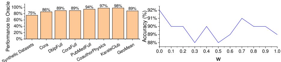
Fig. 9. Performance of our approach related to the Oracle performance. Fig. 10. Prediction accuracy of our approach when varying w in Eq 1.
