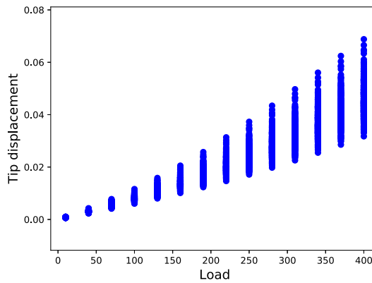
Figure 10. Tip displacement samples generated by the nonlinear cantilever.
