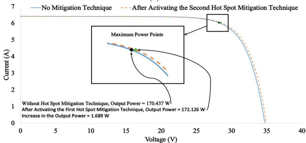
Fig. 9. Photovoltaic output I-V curve. (a) Before and after activating the first hot spot mitigation technique, (b) before and after activating the second hot spot mitigation technique
