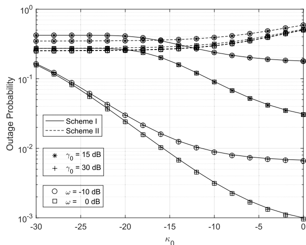
(b) Outage probability versus \kappa_0 with different \gamma_0 and \omega .
