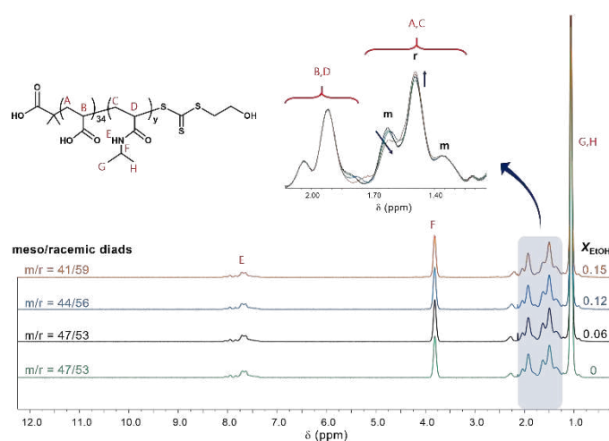
Figure 4. 1 H NMR spectra of purified pAA 34 -b-pNIPAM 184 diblock copolymers synthesised in water and water/EtOH mixtures. The r and m labels are used to denote the resonances attributed to the racemic and meso diads, respectively. Spectra were recorded in D 2 O.
