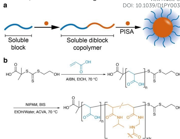
Scheme 1. a) Schematic of the polymerisation-induced self-assembly process.
