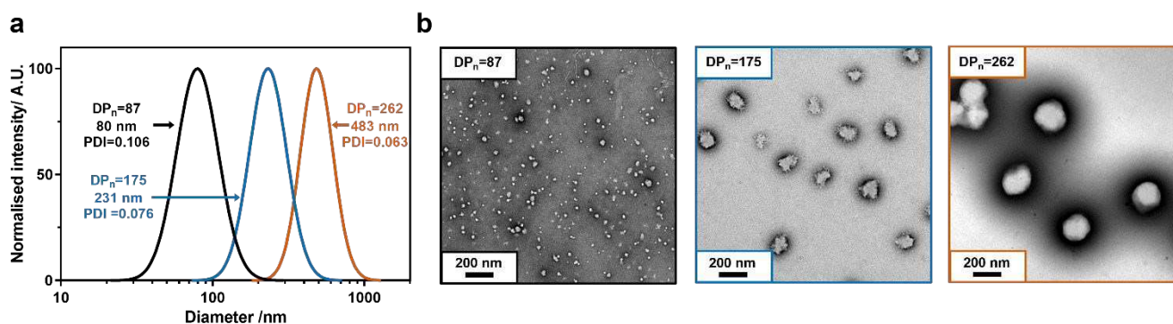
Figure 1. Characterisation of pAA 45 -b-pNIPAM x /BIS 3 ( x = 87, 175 and 262 ) nanogels synthesised in water. a) Intensity average log normal size distributions from dynamic light-scattering. b) Transmission electron micrographs. DP_n indicates the targeted DP of pNIPAM. DLS and TEM samples were prepared from 0.1% w/v nanogel dispersions in water at pH 7 at 25 °C. TEM samples were stained with phosphotungstic acid (0.75% w/v, pH 7).
