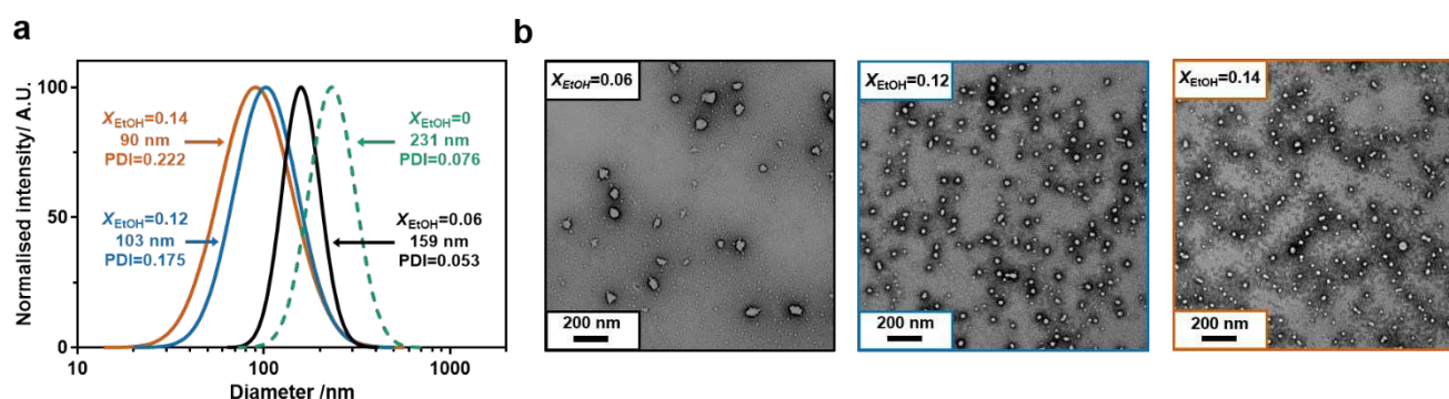
Figure 2. Characterisation of pAA 45 - b -pNIPAM 175 /BIS 3 nanogels synthesised in water/EtOH mixtures. a) Intensity average log normal size distributions from dynamic light-scattering. b) Transmission electron micrographs. DLS and TEM samples were prepared from 0.1% w/v nanogel dispersions in water at pH 7 at 25 °C. TEM samples were stained with phosphotungstic acid (0.75% w/v, pH 7).
