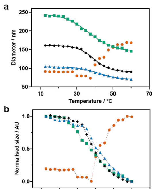
Figure 3. a) Variable temperature DLS data for pAA 45 -b-(pNIPAM 175 /BIS 3 ) nanogels synthesised in water and water/EtOH mixtures. b) Normalised sizes. DLS measurements were obtained from 0.1% w/v nanogel aqueous dispersions at pH 7.
