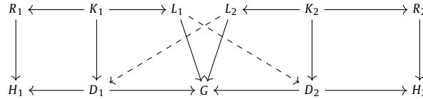
Fig. 3. Parallelly independent direct derivations.
