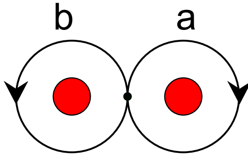
Figure 6: The two elements (a, b) of the free group.
