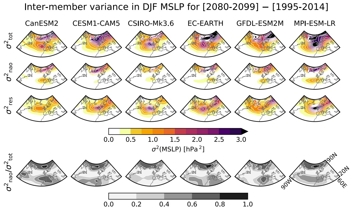
Figure 2. Inter-member variance in projections of December to February (DJF) mean sea level pressure (MSLP) for (2080–2099) – (1995–2014) for each Multimodel Large Ensemble Archive (MMLEA) model. (Top row) Total ( \sigma^2_{\text{tot}} ); (Second row) North Atlantic Oscillation (NAO)-congruent part ( \sigma^2_{\text{nao}} ); (Third row) Residual ( \sigma^2_{\text{res}} ); (Bottom row) Proportion of total variance explained by NAO. \sigma^2_{\text{nao}} is obtained by regressing the total intermember spread in MSLP on the spread in NAO-congruent MSLP at each grid-point. \sigma^2_{\text{res}} is the variance in the residuals of this regression.
