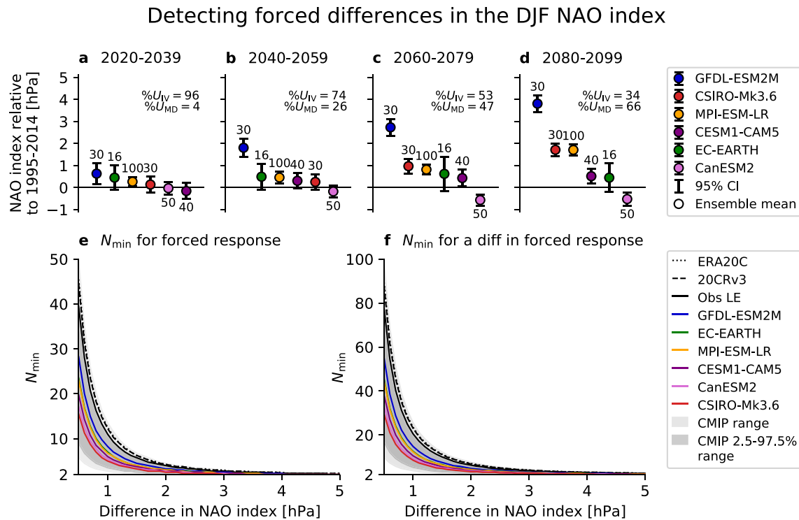
Figure 3. Detecting a forced response in December to February (DJF) North Atlantic Oscillation (NAO) index and inter-model differences in this response. (a–d), NAO anomalies in Multimodel Large Ensemble Archive (MMLEA) models for future 20-year epochs (1995–2014 baseline). Whiskers are 95% confidence intervals and numbers indicate ensemble size. Section 2.3 defines \%U_{IV} and \%U_{MD} . (e), N_{\min} required to detect a forced NAO response of a given magnitude at the 95% confidence level based on IV estimates from MMLEA models, CMIP5/6 models, and observation-based datasets (Text S2 and S3). (f), As in (e) but for detecting a difference in forced response; note different y-axis scale. Single CMIP5/6 models can be located within the gray plumes using Table S2.
