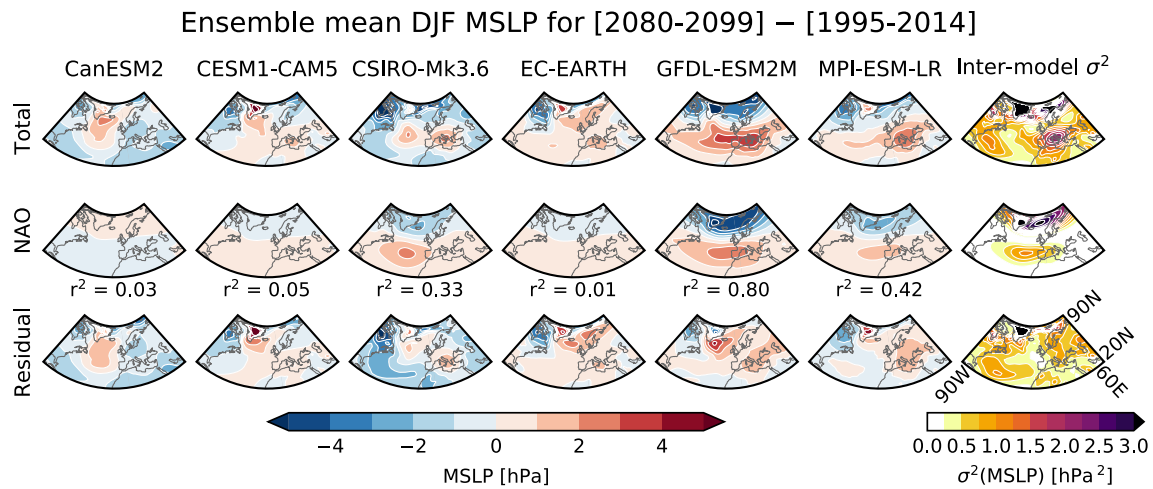
Figure 4. Projections of ensemble mean December to February (DJF) mean sea level pressure (MSLP) for (2080–2099) – (1995–2014) for each Multimodel Large Ensemble Archive (MMLEA) model, and their inter-model variance. (Top) Total; (Middle) North Atlantic Oscillation (NAO)-congruent part; (Bottom) Residual. r^2 is the squared area-weighted pattern correlation between the total response and the NAO-congruent part.
