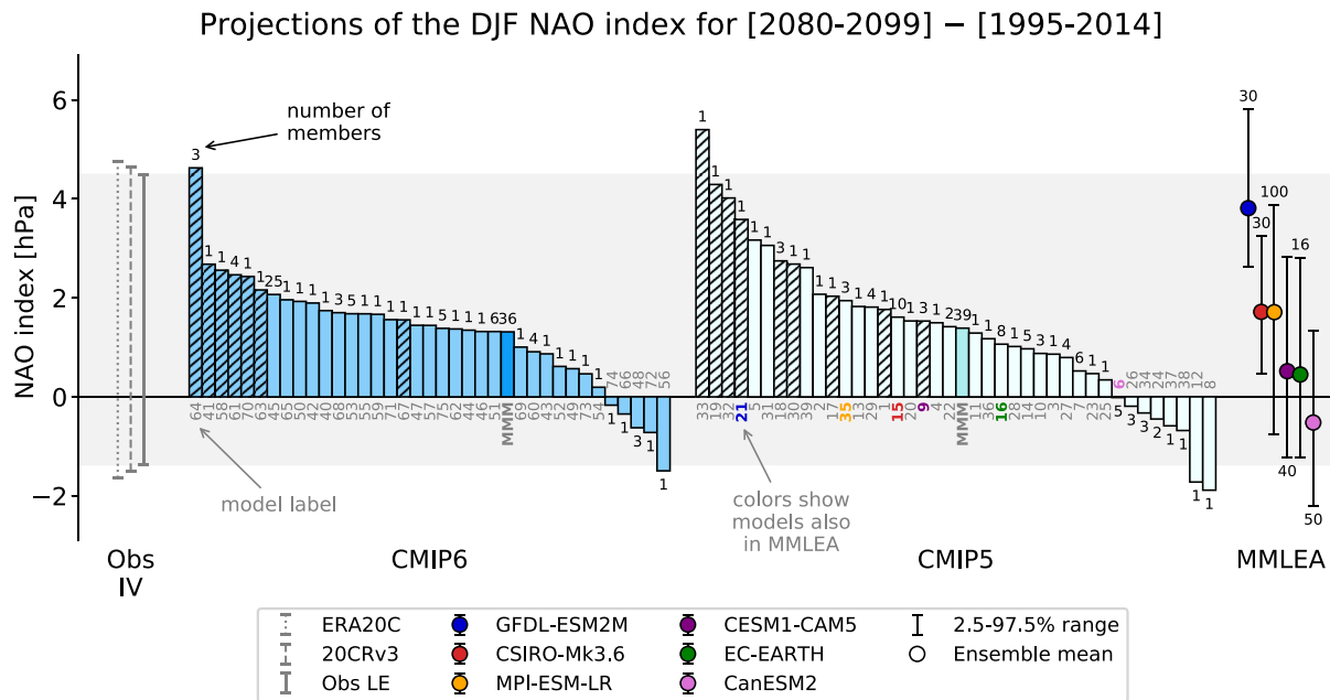
Figure 1. Projections of the December to February (DJF) North Atlantic Oscillation (NAO) index for (2080–2099) – (1995–2014) in the CMIP6, CMIP5, and Multimodel Large Ensemble Archive (MMLEA) models. For CMIP5/6 models, ensemble means are shown if more than one ensemble member is available. Hatching indicates a CMIP5/6 model anomaly that is larger than 2 standard deviations of model-specific internal variability (IV) (Text S3). Darker cyan/blue bars indicate the multimodel mean (MMM). Whiskers for MMLEA models indicate the 2.5%–97.5% range of responses across the ensemble members. Section 2.1 describes the model forcing scenarios. Gray lines show the 2.5%–97.5% range of 10^3 differences in 20-year epoch means of different observation-based records (Section 2.1), selected by randomly resampling with replacement. Gray shaded box shows this range for Obs LE. The observation-based IV estimates are shifted by the CMIP6 MMM anomaly for comparison with the inter-model spread.
