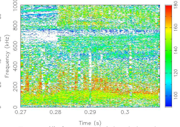
Figure 1(f) \Theta_H > 90^\circ : left-handed modes
