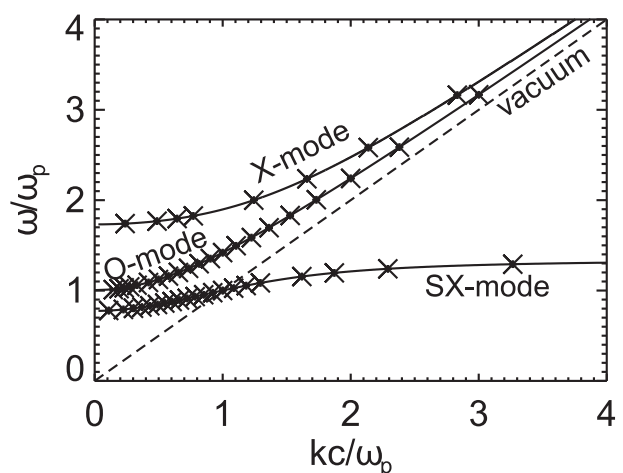
Figure 1: Dispersion relation of the O- and X-mode as obtained from simulations (crosses) and cold plasma theory (solid lines).
