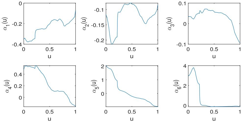
Figure 4. Post-clustering estimates of the functional coefficients in Example 6.1 with \alpha_k(\cdot) , for each k = 1, 2, \dots, 6 , being the estimated functional coefficient corresponding to the k th cluster listed in Table 10.
