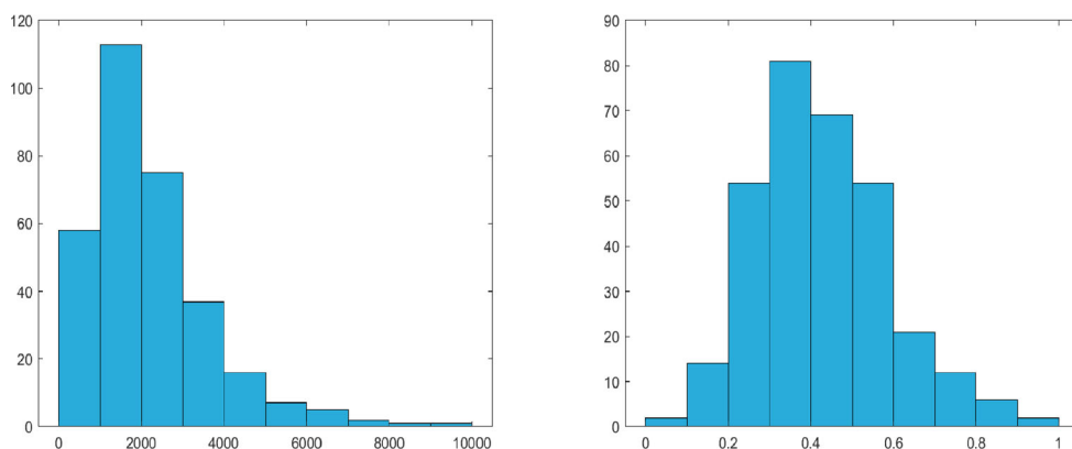
Figure 6. Histograms for the original and transformed index variable in Example 6.2. Left panel: original data for BETADIET, right panel: BETADIET after the square-root and min-max transformations.
