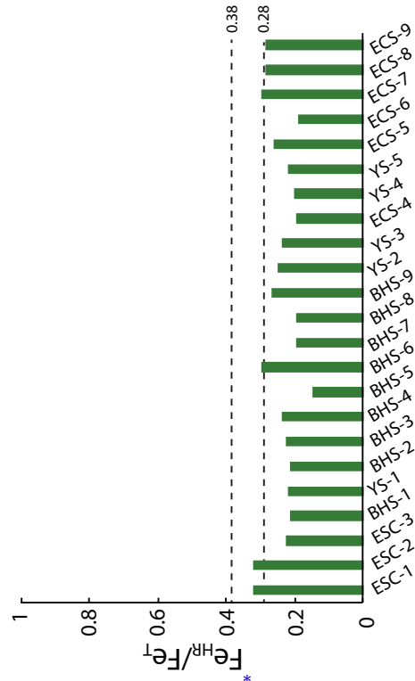
B. Fe_{HR} for the Bohai, Yellow Sea and East China Sea sediments
