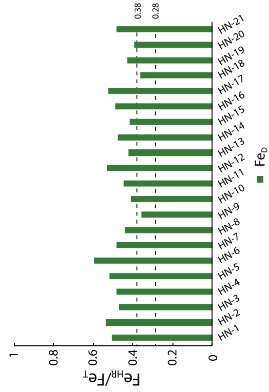
D. Fe_{HR} for the Hainan offshore sediments
