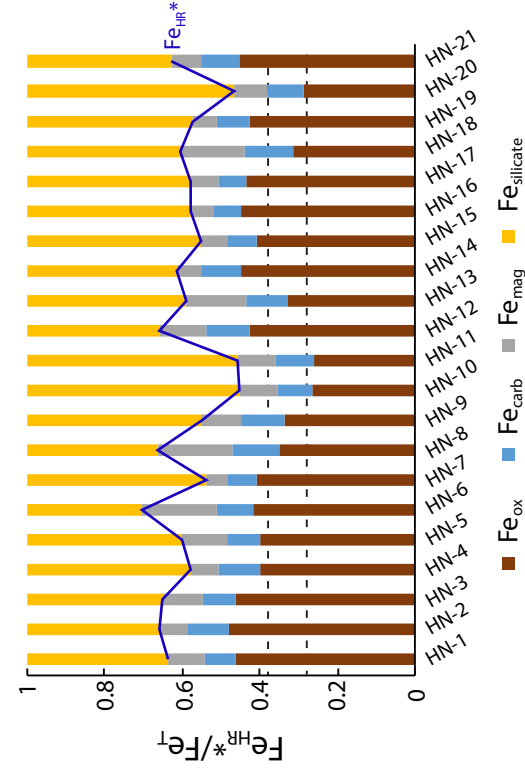
C. Fe_{HR}^* for the Hainan offshore sediments
