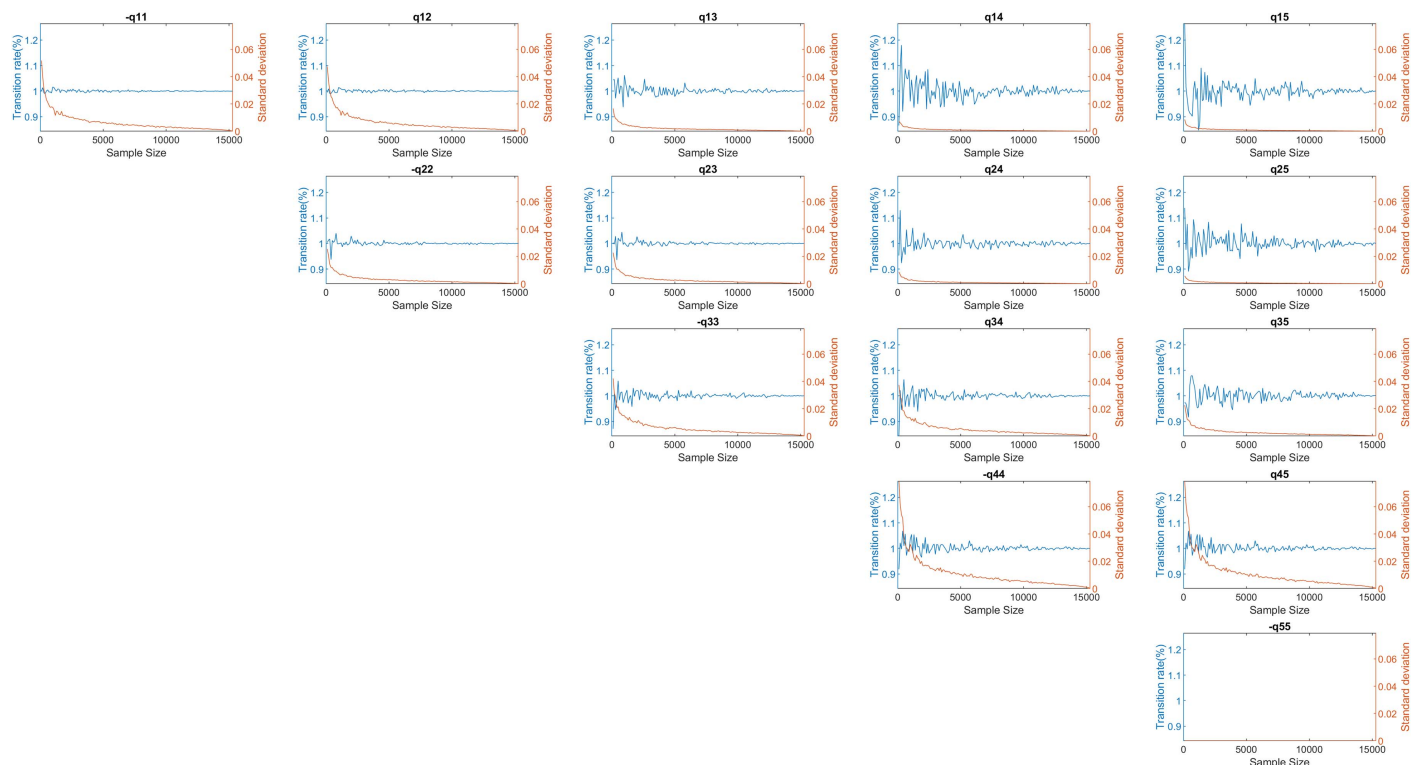
Fig. 1. Mean and standard deviation of transition rate matrix Q as sample number increases.
