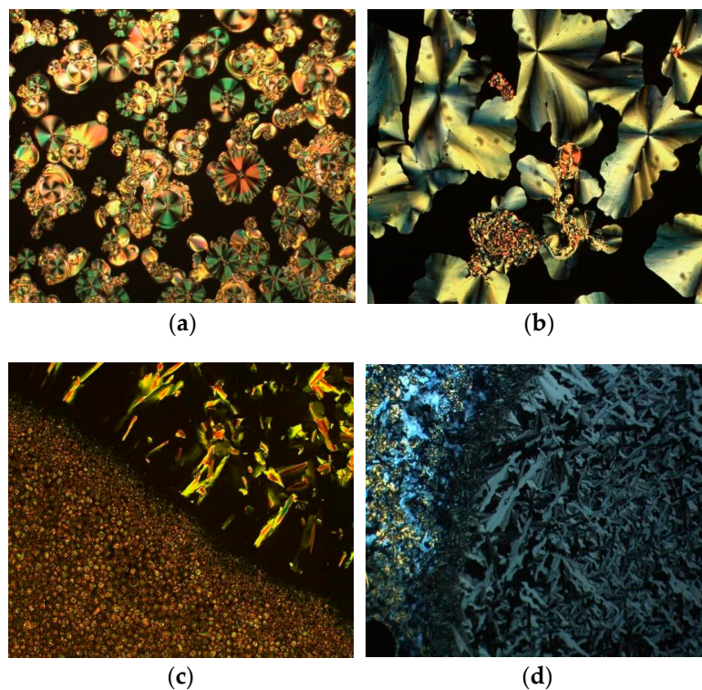
Figure 8. Photomicrographs of the Col r phase formed by compound 5-8: (a) cooling from the isotropic liquid at 10 \text{ }^{\circ}\text{C min}^{-1} at 158 \text{ }^{\circ}\text{C} , (b) slow cooling of the same compound at 0.1 \text{ }^{\circ}\text{C min}^{-1} at 159 \text{ }^{\circ}\text{C} , (c) miscibility gap between this phase and the Col h phase of the OTf compound 1-18 (5-8 is bottom left and 1-18 is top right) and (d) miscibility gap between the phase of 5-8 (top and left) and the SmA phase of the OTf compound 1-12 (right).
