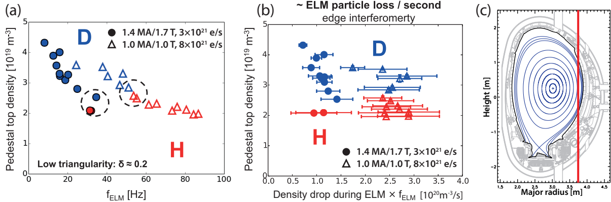
Figure 10. (a) n_{\text{e,PED}} as a function of f_{\text{ELM}} in low \delta(=0.2) H (red) and D (blue) plasmas at 1.4 MA/1.7 T (full circles) and 1.0 MA/1.0 T (open triangles). H and D pedestals at similar f_{\text{ELM}} (but different P_{\text{sep}} ) have comparable pedestal densities as highlighted by the black dashed circles. (b) n_{\text{e,PED}} as a function of average drop in edge interferometer signal during ELMs per second. The error bars represent the statistical variation of the ELM particle loss throughout the steady phase of the discharge. (c) The line-of-sight of the edge interferometry channel (in red) used for the ELM particle loss analysis in a poloidal cross-section of JET-ILW.
