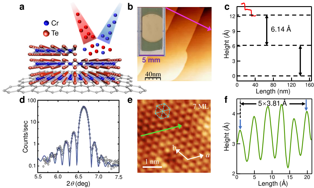
Fig. 1 Crystal structure and STM characterizations of epitaxially grown \text{CrTe}_2 thin films. a Schematic illustration of MBE growth process of \text{CrTe}_2 films on graphene. b The STM topology image ( 200 \times 200 \text{ nm}^2 ) of a 7 ML \text{CrTe}_2 fabricated on graphene/SiC. U = +1 \text{ V} , I_t = 200 \text{ pA} . Inset on the left is an optical image. c The line-scan profile taken along the pink line in b , with an average step height of \sim 6.14 \text{ \AA} . d XRD spectrum showing Laue fringes around the (001) \text{CrTe}_2 reflections. The solid fitting curve indicates the thickness of 39 layers, the roughness of 2 layers and the lattice constant c = 6.13 \text{ \AA} . e Atomically resolved STM image ( 4 \times 4 \text{ nm}^2 ) with a hexagonal structure. U = -1.5 \text{ mV} , I_t = -440 \text{ pA} . f The line-scan along the green arrow in e , showing a lattice periodicity of \sim 3.81 \text{ \AA} .
