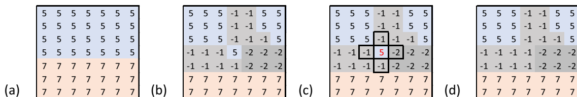
Fig. 6. Segmentation-cleaning; (a): Initial segmentation; (b): After mask application; (c): Detection of isolated pixels; (d): Replacement of isolated pixels with the most common value of the 3 × 3 ROI (limited to 4-connectivity labels).
