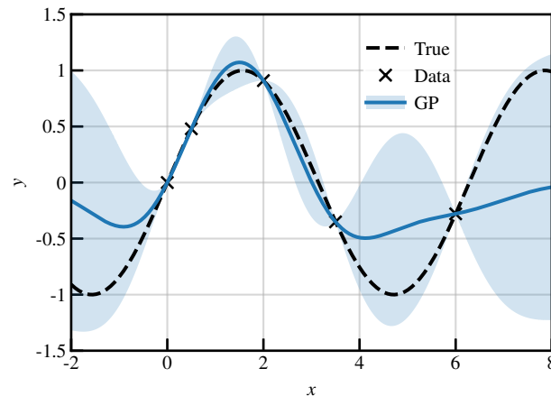
Figure 2. Demonstration of Gaussian process regression. The true function is y = \sin(x) , and the data points are at x = \{0, 0.5, 2, 3.5, 6\} . The solid line represents the GP mean, and the shaded areas give the 2\sigma confidence intervals. The optimised kernel parameters are \eta^2 = 0.602 , \ell = 1.063 . See text for details.
