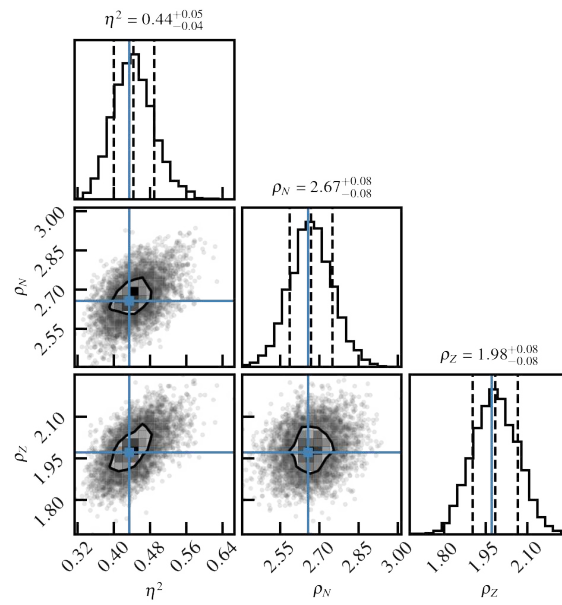
Figure 4. Posterior distributions of GP parameters obtained through MCMC sampling. The horizontal and vertical solid lines indicate the optimal parameter values obtained by maximising the likelihood. The vertical dotted lines on each 1D histogram indicate the mean and 1\sigma confidence intervals obtained through MCMC sampling. See text for details.
