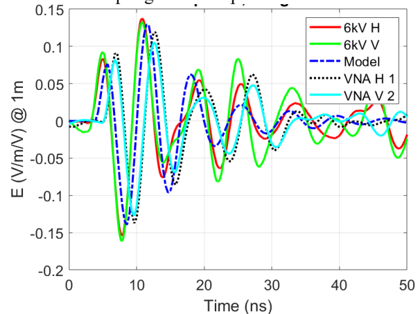
Fig. 3. Comparing Dipole antenna numerical model results with VNA and pulse measurement
