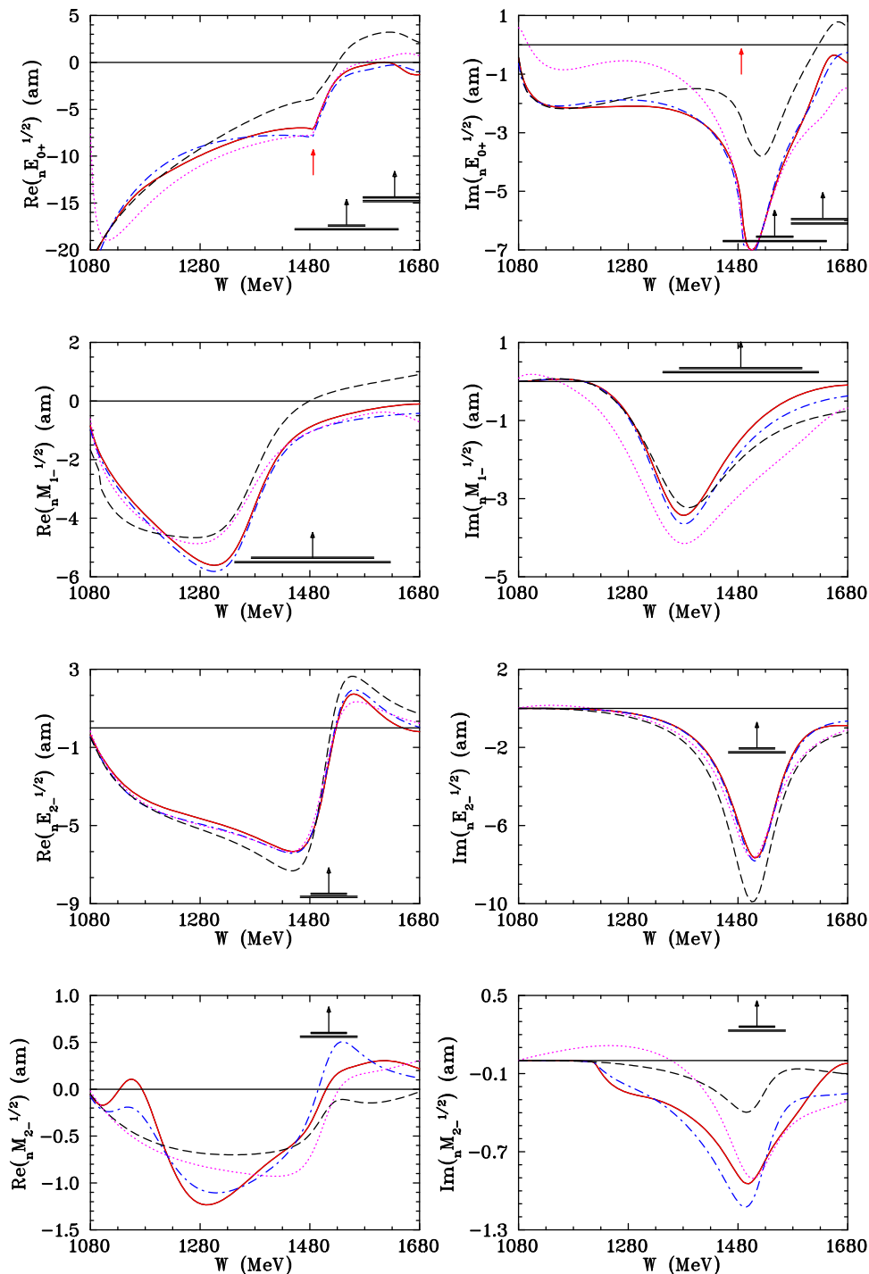
Fig. 9 Selected neutron multipole I = 1/2 amplitude from threshold to W = 1.68 GeV ( E_\gamma = 1030 MeV) for the states 0^+ , 1^- and 2^- . The blue dash-dotted (red solid) curves correspond to the SAID MA19 [3] (new MU22 including present A2 data) solution. The magenta dotted (black dashed) curves give the Bonn–Gatchina BG2014-02 [28] (MAID2007 [29]). The vertical black arrows indicate Breit–Wigner (BW) mass ( W_R ), and horizontal bars show full ( \Gamma ) and partial ( \Gamma_{\pi N} ) widths of resonances extracted by the BW fit of the \pi N data associated with the SAID solution SP06 [32]. Vertical red arrows show the \eta meson production threshold
