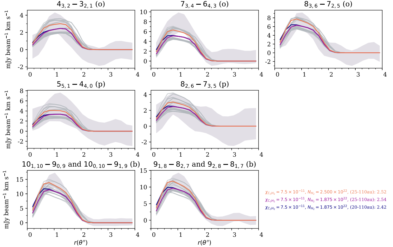
Figure 6. Radial profiles of the integrated emission from each transition, including error bars (shaded gray). Profiles extracted using GoFish. The thirty best fit models are shown as gray lines, while the top three models are shown in color, and have parameters indicated in the legend in the lower right-hand corner.
