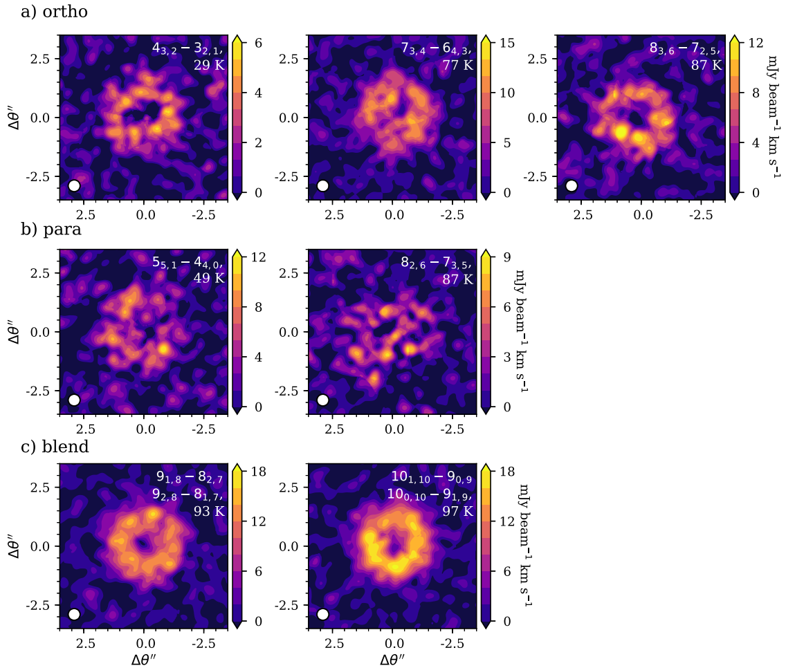
Figure 1. Moment zero maps for the five isolated transitions of a) ortho, b) para, and c) two blended transitions of c\text{-C}_3\text{H}_2 that are analyzed in this work. Line ID and upper state energy are labelled in the upper right corner of each panel.
