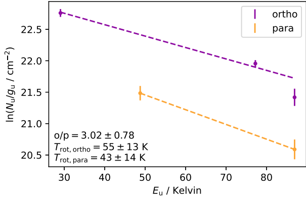
Figure 7. Disk-averaged rotational diagram of the unblended lines. We find similar ortho and para rotational temperatures and a disk integrated ortho-to-para ratio consistent with 3.
