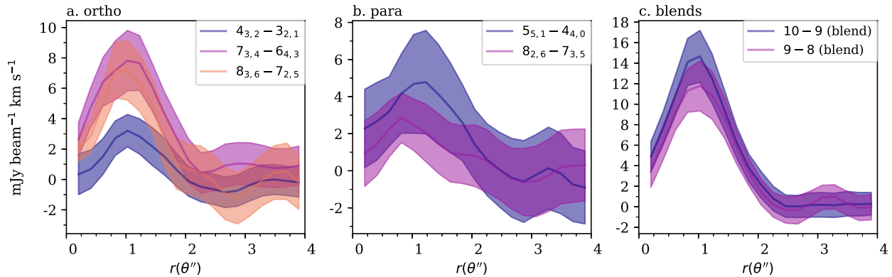
Figure 2. Profiles extracted by the pixel stacking technique within the GoFish code (Teague 2019). Transitions indicated in the legend. Shaded region indicates the error on the radial profile.
