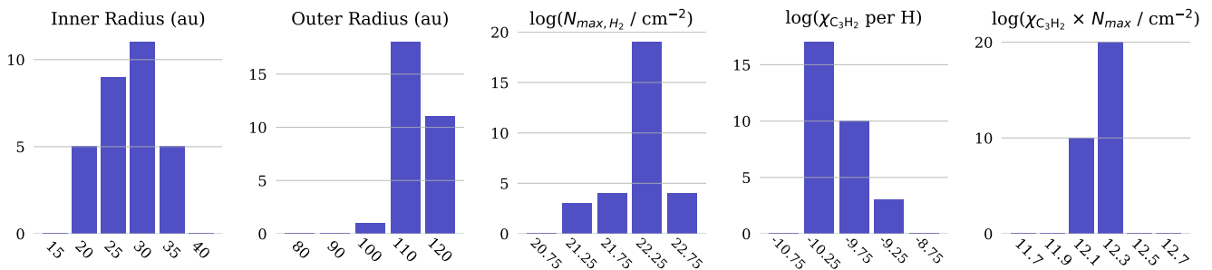
Figure 5. Histogram of the parameters of the 30 best fit models. Note 1 A_V corresponds to N_{\text{H}_2} = 1.27 \times 10^{22} \text{ cm}^{-2} given the reduced dust in the upper layers of TW Hya.
