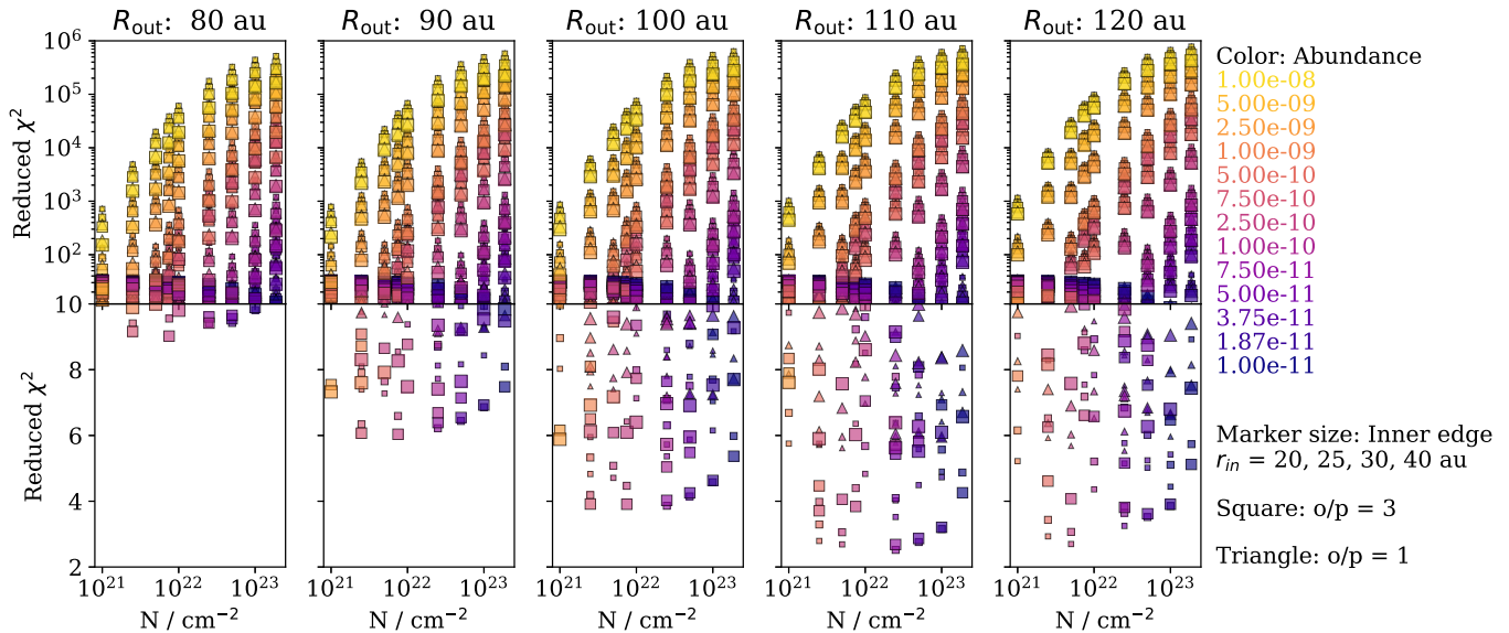
Figure 4. Reduced \chi^2 between the observed visibilities and modelled visibilities. Each point represents the model fit for all observed lines as a summed reduced \chi^2 . The model parameters are described by the point color (abundance), size (inner radius of c\text{-C}_3\text{H}_2 ), and shape (ortho to para ratio). The columns indicate different outer radii for the c\text{-C}_3\text{H}_2 slab, for the full range of \text{H}_2 column densities considered on each x-axis. The poor fits are shown on a logarithmic scale on the top row, while the better fits are shown as a linear scale on the bottom row.
