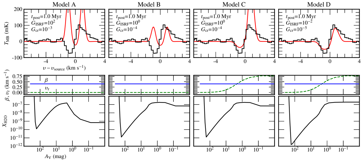
Fig. 20. Illustration how various physical and chemical parameters can be constrained using the SWaN network. \text{H}_2\text{O } 1_{01} - 1_{01} 557 GHz observations of the Class I source L1551-IRS5 are compared with SWaN models assuming different parameters for the FUV fluxes and velocity profile. The top row shows the observations (black) together with the synthetic spectra (red), whereas the bottom row shows the adopted velocity profile (green) and water abundance profile (with respect to \text{H}_2 ) (black). A constant Doppler broadening of \beta=0.4 \text{ km s}^{-1} is assumed, whereas the radial velocity profile is either taken to be constant at 0 (Models A and B) or to have an expansion profile (Models C and D). The radiation fields G_{\text{ISRF}} and G_{\text{CR}} strongly decrease from model A to model D. A pre-stellar stage duration of 0.1 Myr is used. Based on Schmalzl et al. (2014).
