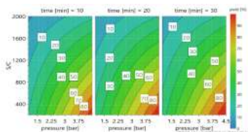
Figure S11. Results of Screening by DoE
