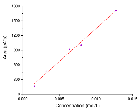
Figure S21. racemic methyl 3-acetamidobutanoate calibration curve
