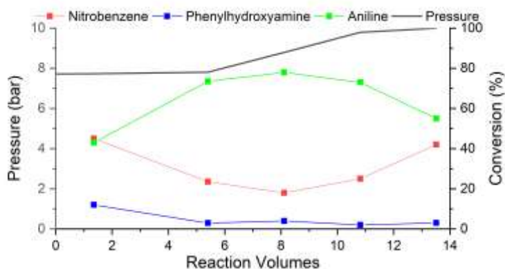
Figure S15. Continuous Hydrogenation of Nitrobenzene Entry 25
