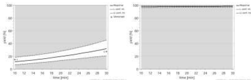
Figure S12. Predicted kinetic profiles of the reaction constituents of S/C = 2000 (left) and S/C = 200 (right) in 4.5 bar.
