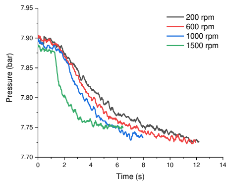
Figure S5. The pressure changing under different stirring rates with 1 mL MeOH ( r = 0.7 ) in the reactor
