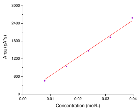
Figure S7. Nitrobenzene calibration curve
