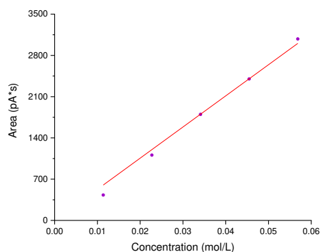
Figure S8. Aniline calibration curve
