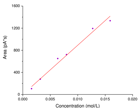
Figure S20. (E)-methyl-3-acetamido-2-butenoate calibration curve
