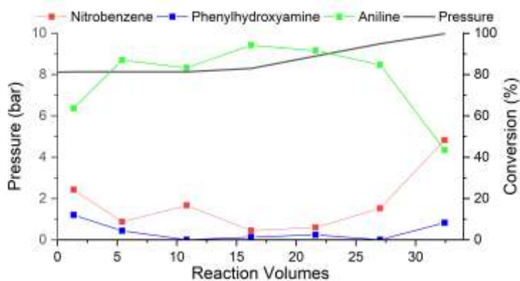
Figure S14. Continuous hydrogenation of nitrobenzene Entry 24
