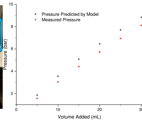
Figure S4. Left (a) Adding pressure by a 5 mL syringe pump; Right (b) prediction and measured value.
