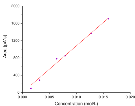
Figure S19. ( Z )-methyl-3-acetamido-2-butenoate calibration curve
