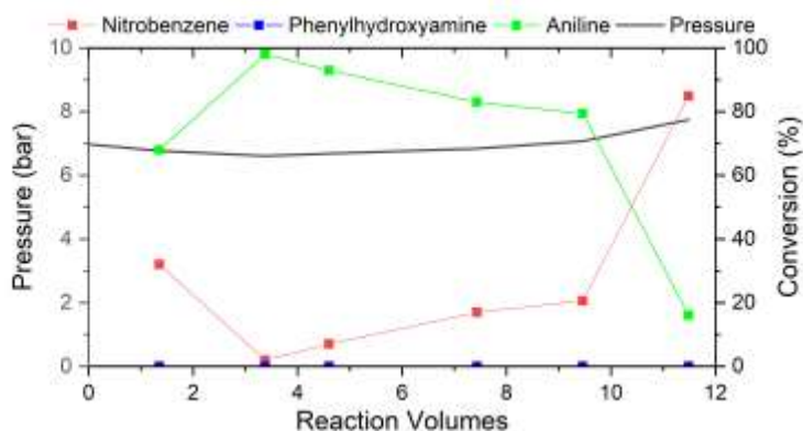
Figure S16. Continuous Hydrogenation of Nitrobenzene Entry 26
