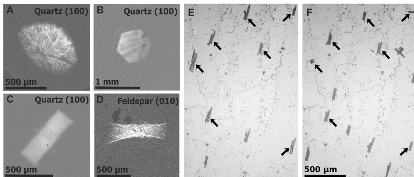
Fig. 2. Optical micrographs from immersion freezing and deposition experiments. ( A–D ) Immersion ice freezing showing ( A ) spherical, ( B ) hexagonal, and ( C ) rectangular morphology on the quartz (100) face and ( D ) rectangular morphology on the feldspar (010) face. Images are obtained by subtraction from an image just prior to nucleation. Note that in all cases, the growing crystal is a large number of narrow dendrites rather than a continuous solid. ( E and F ) Deposition ice growth on (010) feldspar on two consecutive cycles on the same region. Black arrows indicate sites that produced an ice crystal on both cycles. Note that images in both modes have been cropped and that the experimental fields of view were much larger.
