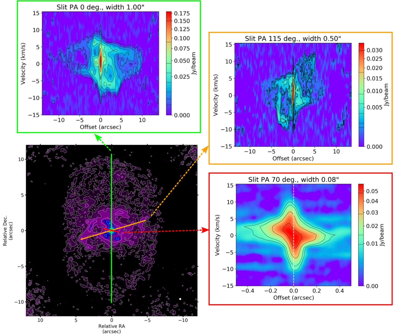
Fig. 8: Bottom-left : Central channel of the LR CO cube, with color-coded symmetry axes obtained from the analysis in Sect. 4.1. The colour-coded encased panels represent the PV diagrams constructed along their respective colour-coded axes. The orientation and width of the slits are specified in each PV panel. Velocities are corrected to the systemic velocity of -10.1 \text{ km s}^{-1} .
