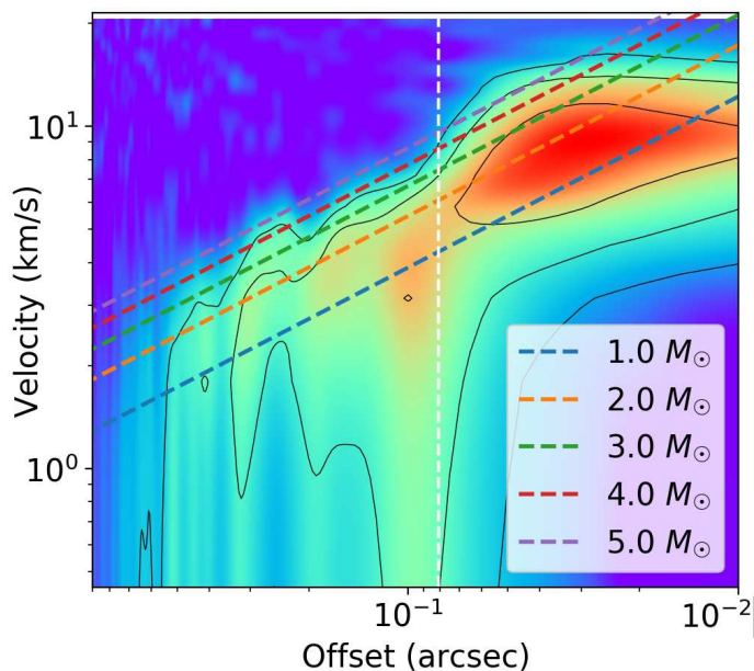
Fig. 14: First quadrant of the PV diagram of the extended SiO data (Fig. 11, right panel) in log-scale. The dotted lines represent Keplerian trends for the respectively color-coded central masses. The vertical, white dashed line represents the position of the ring of compact SiO emission shown in Fig. 13, which is assumed to be the inner rim of the disk. The offset is measured with respect to the stellar position. The contours are drawn at 3, 6, 24 times the noise rms. At offsets larger than the inner rim position, the 3\times\sigma_{\text{rms}} contour lies between the 2 and 4 M_{\odot} Keplerian trends, following the 3 M_{\odot} trend quite closely.
