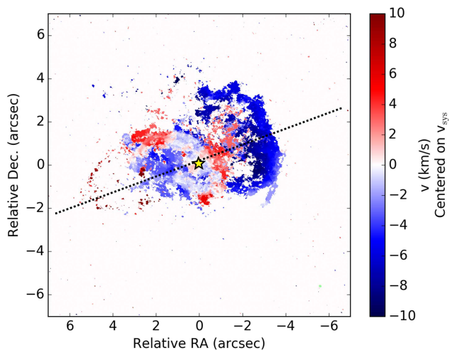
Fig. 7: Moment 1 map of the HR CO data. The dashed line represents the alignment axis separating the eastern and western bubble, which has a position angle of \sim 115^\circ (see also orange line in Fig. 8). The continuum peak is indicated by a yellow star. The tiny green ellipse in the bottom right corner is the ALMA beam.
