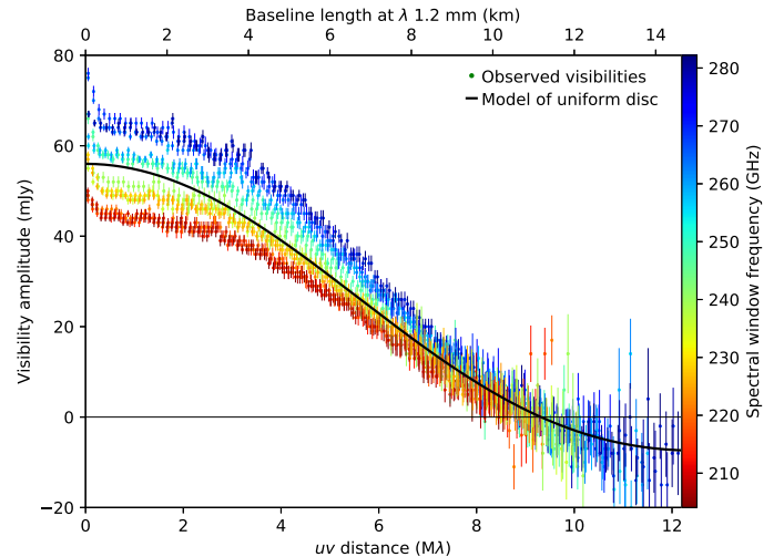
Fig. 2: The continuum observed visibility amplitudes (plotted in colour for each of the 16 spectral windows) as a function of uv distance and the corresponding baseline length. The black line shows the fitted model for a uniform disc of radius 13.5 milliarcseconds and flux density 56 mJy. See text for more details.
