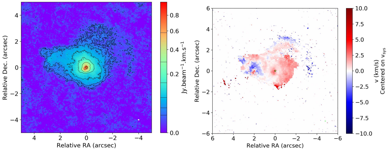
Fig. A.6: Left : Moment0 map of the SiO v=0 J=5-4 emission. Contours are drawn at 3, 6, 12, 24, 48, 96, and 192 times the rms noise value in the spectral region of the bandpass without detectable line emission ( \sigma_{\text{rms}} = 8.0 \times 10^{-4} Jy/beam). Right : Moment1 map of the same emission.
