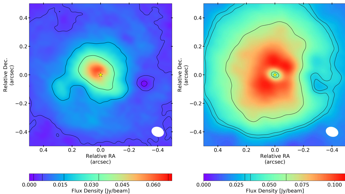
Fig. 15: The channel maps where an unresolved emission void is detected about 0.3'' to the west of the AGB star (indicated by the yellow star). Left : CO, channel at 0.5 \text{ km s}^{-1} , contour levels [3,9,24,48,96] \times \sigma_{\text{rms}} . Right : SiO, channel at 0.6 \text{ km s}^{-1} , contour levels [46,51,90] \times \sigma_{\text{rms}} . The contour levels have been chosen to highlight the feature.
