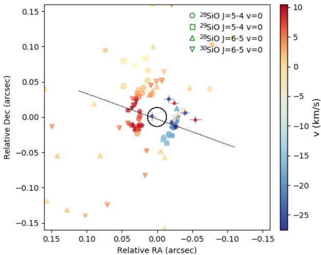
Fig. 13: Same as Fig. 12, but for the extended configuration dataset. Note that the velocity scale differs from Fig. 12.
