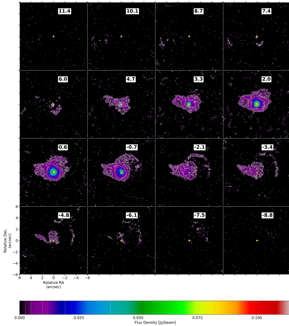
Fig. 10: Channel maps showing the spatially resolved emission of the SiO v=0 J=5-4 line in the \pm \sim 10 km s ^{-1} velocity range, for the combined dataset. The velocities have been corrected for v_*=-10.1 km s ^{-1} . Contours are drawn at 3, 6, 12, 24, 48, 96, and 192 \times \sigma_{\text{rms}} ( \sigma_{\text{rms}} = 0.7 \times 10^{-3} Jy/beam). Angular scales are indicated in the bottom left panel. The ALMA beam has a size ( 0.088'' \times 0.066'' ). The maps are centred on the continuum peak at position (0,0), and are indicated by a tiny yellow star.
