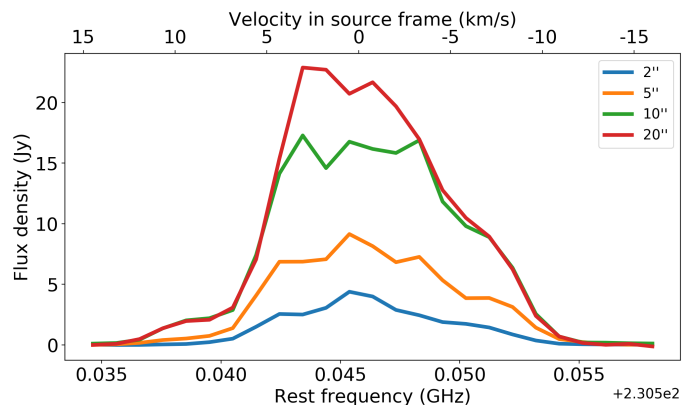
Fig. 3: Spectrum of the CO v=0 J = 2-1 , LR cube, obtained for different extraction aperture diameters. The frequency axis is adjusted to the stellar velocity. The overbar marks the LSR velocity of the star.
