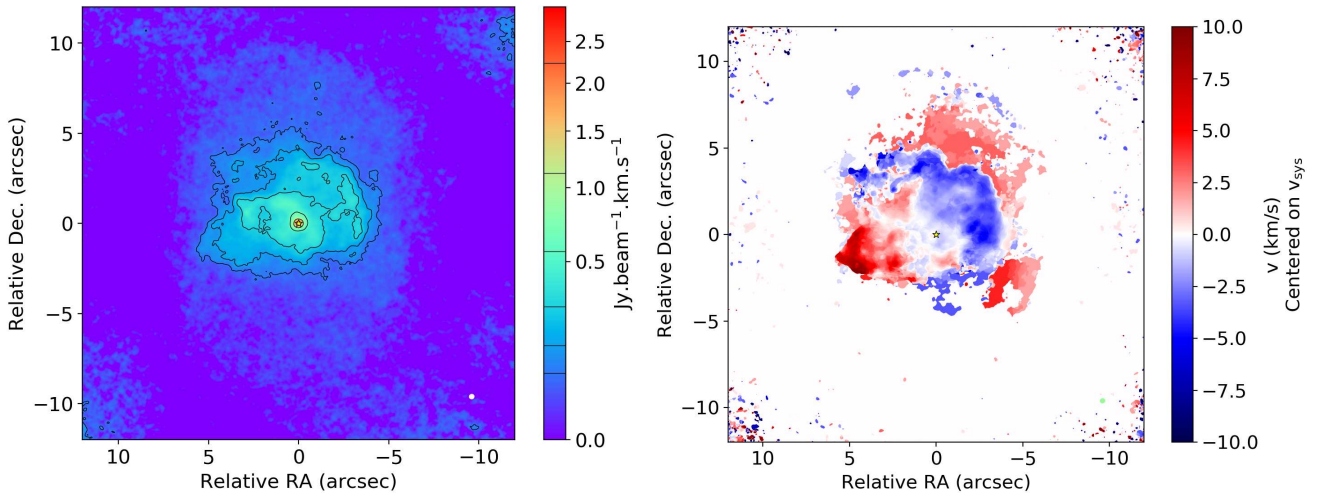
Fig. A.3: Moment0 ( left ) and moment1 ( right ) maps of the LR CO emission in the channel maps shown in Fig. 4. Contours are drawn at 3, 6, 12, 24, 48, and 96 times the rms noise value in the spectral region of the bandpass without detectable line emission. The continuum peak position is indicated by the yellow star.
