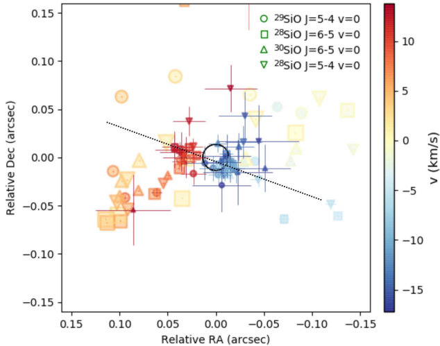
Fig. 12: Position and velocity of the peak positions of the Gaussian-fitted components of the ^{28}\text{SiO} , ^{29}\text{SiO} J = 5-4 and ^{28}\text{SiO} , ^{30}\text{SiO} J = 6-5 ground-state vibrational emission lines of the mid-configuration dataset. The black circle in the middle represents the size of the stellar photosphere (Sect. 3). The marker size reflects the magnitudes of the integrated flux of the Gaussian-fitted component, scaled as \log_{10}(\text{integrated flux}) . The dashed black line indicates the \text{PA}=70^\circ axis.
