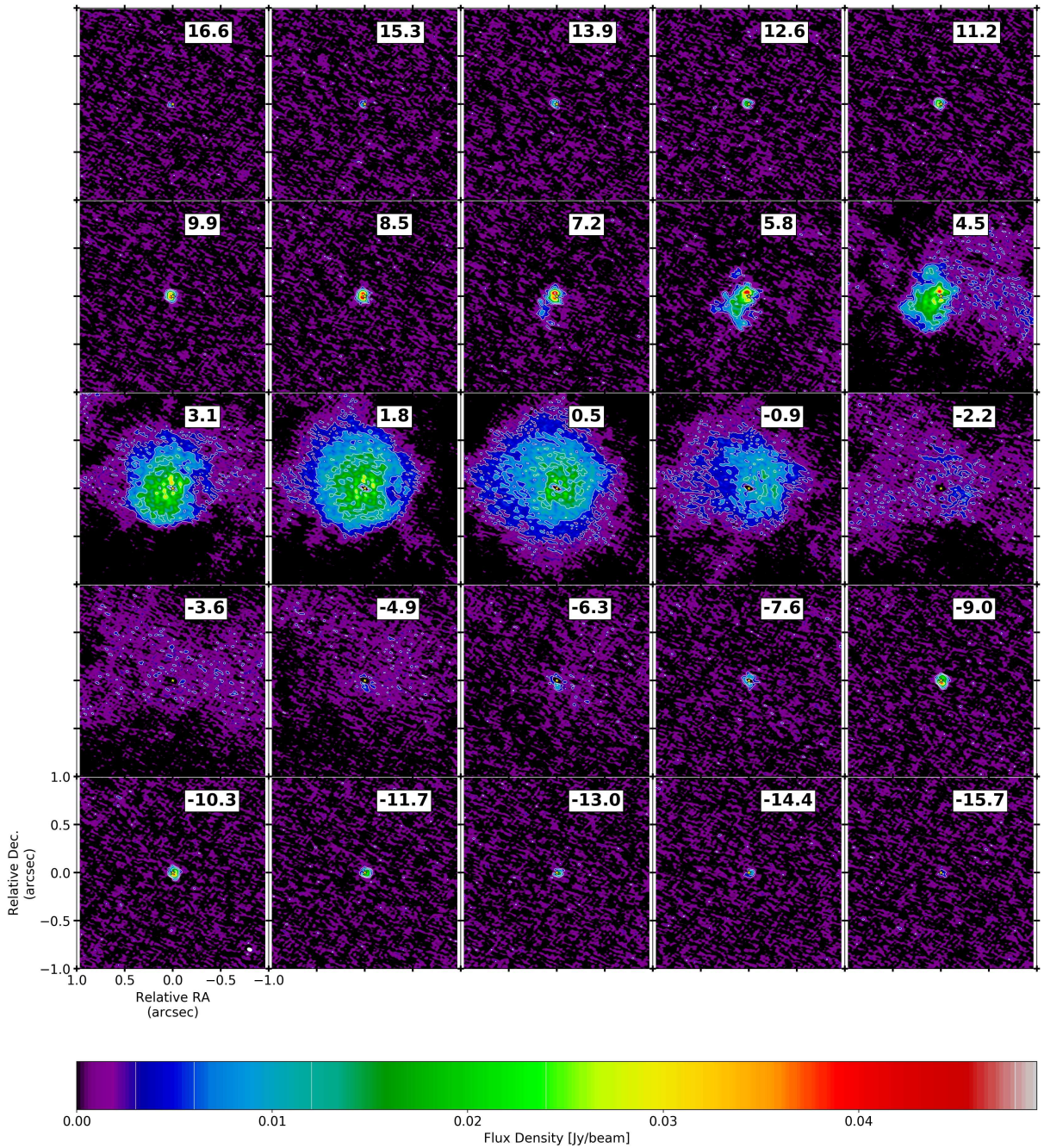
Fig. A.5: Channel maps showing the spatially resolved emission of the SiO v=0 J = 5-4 , for the extended dataset. The velocities have been corrected for v_* = -10.1 km s ^{-1} . Contours are drawn at 3, 6, 12, 24, 48, 96, and 192 \times \sigma_{\text{rms}} ( \sigma_{\text{rms}} = 1 \times 10^{-3} Jy/beam). The ALMA beam has a size of (0.047'' \times 0.03'') . Angular scales and are indicated in the bottom left panel. The maps are centred on the continuum peak at position (0,0), indicated by a tiny yellow star.
