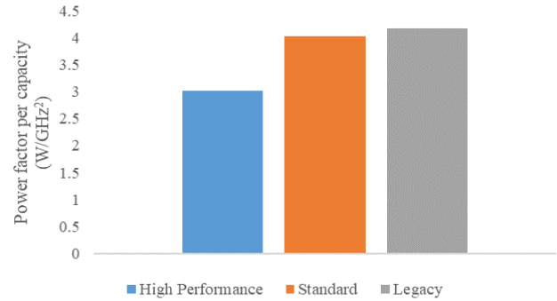
Fig. 6. Power factor per capacity of server CPU components
