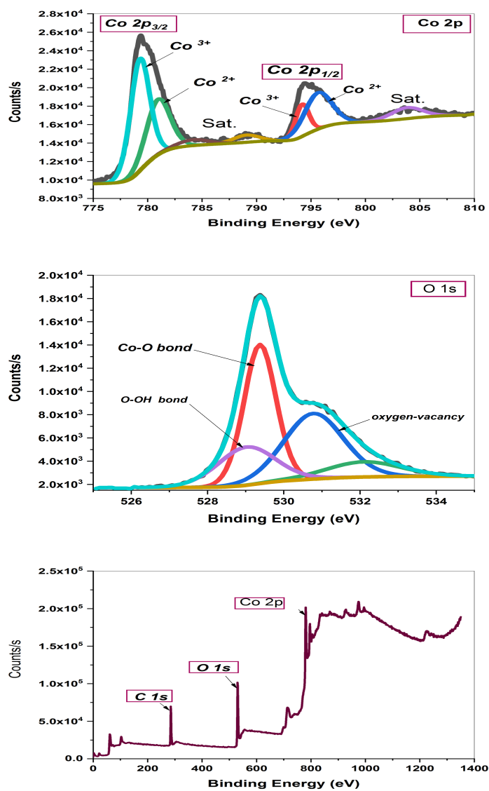
Figure 6:- XPS spectra of pure Co 3 O 4 film.
