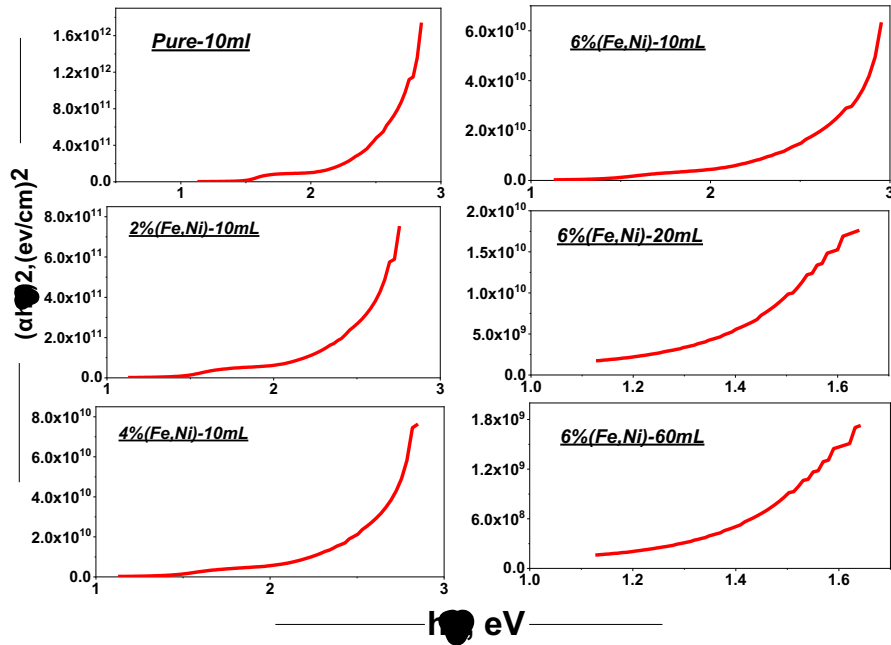
Fig. 4. Variation of (\alpha hv)^2 versus hv for all deposited films to calculate the bandgap.
