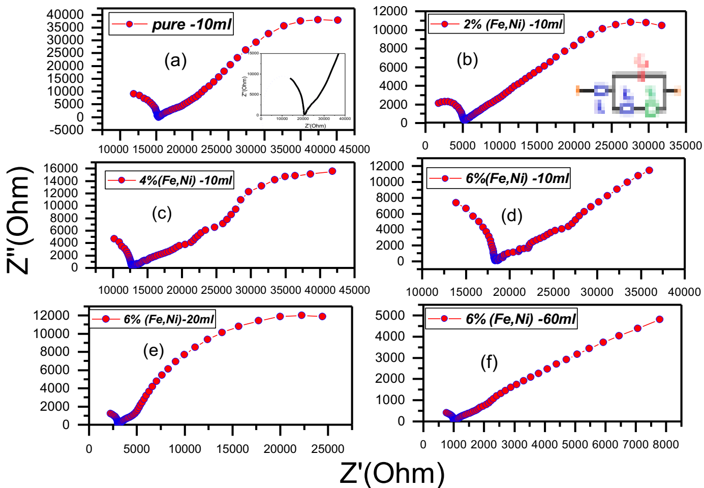
Fig. 10. Nyquist plots for pure and (Fe, Ni) codoped \text{Co}_3\text{O}_4 photoelectrodes in 0.3 M \text{Na}_2\text{SO}_4 electrolyte at 0V (vs Ag/AgCl) and under white light illumination.
