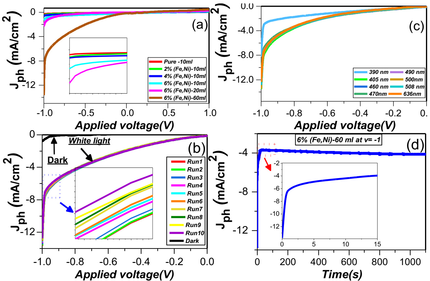
Fig. 7. Variation of J_{ph} versus the applied voltage for (a) all photoelectrodes under white light illumination, (b) 6%(Fe, Ni)-60ml Co 3 O 4 photoelectrode for a different number of runs under dark and white light illumination conditions, and (c) 6%(Fe, Ni)-60ml Co 3 O 4 photoelectrode under monochromatic illumination; and (d) J_{ph} versus exposure time for 6%(Fe, Ni)-60ml Co 3 O 4 photoelectrode at -1V.
