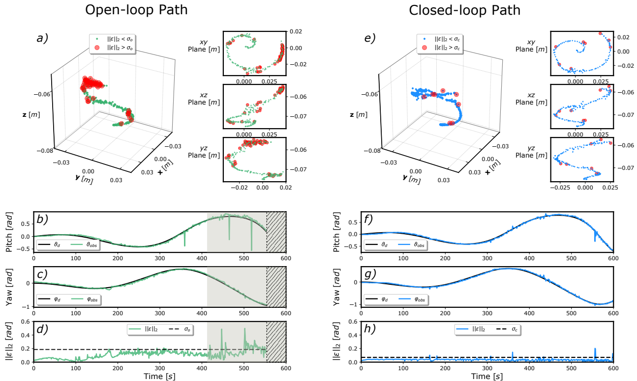
Figure 9. Path following results for open-loop (left column) and closed-loop (right column) strategies applied to the HydroJet soft continuum manipulator under TFA with the base oriented parallel to Earth's surface, such that gravity acts along the z -axis of the robot at its base (0 degrees base angle). Graphs a) and e) show a 3D view of the measured path followed by the capsule-shaped tip and its projection on xy , xz and yz planes for open-loop and closed-loop, respectively; the red dots indicate the locations of points on the path where the norm of the error was greater than a pre-defined threshold ( \sigma = 90^{th} -percentile). The desired (black line) and measured (colored lines) paths for pitch and yaw angles are shown in b) and c) for the open-loop case, and in f) and g) for the closed-loop case. Finally, the norm of the error is presented for open-loop and closed-loop trials in d) and h), respectively; the threshold (dashed line) representing the 90^{th} -percentile, the region where the tip oscillations become large (shaded region), and areas where the trial was aborted due to excessive oscillations ( \vartheta > 0.5 rad) (shaded region with hatch) are shown.
