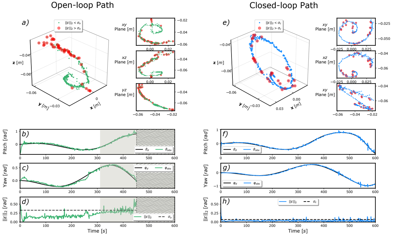
Figure 10. Path following results for open-loop (left column) and closed-loop (right column) strategies applied to the HydroJet soft continuum manipulator under TFA with the base in a bent configuration with respect to gravity (30 degrees base angle). Graphs a) and e) show a 3D view of the measured path followed by the capsule-shaped tip and its projection on xy , xz and yz planes for open-loop and closed-loop, respectively; the red dots indicate the locations of points on the path where the norm of the error was greater than a pre-defined threshold ( \sigma = 90^{th} -percentile). The desired (black line) and measured (coloured lines) paths for pitch and yaw angles are shown in b) and c) for the open-loop case, and in f) and g) for the closed-loop case. Finally, the norm of the error is presented for open-loop and closed-loop trials in d) and h), respectively; the threshold (dashed line) representing the 90^{th} -percentile, the region where where the tip oscillations become large (shaded region), and areas where the trial was aborted due to excessive oscillations ( \vartheta > 0.5 rad (shaded region with hatch) are shown.
