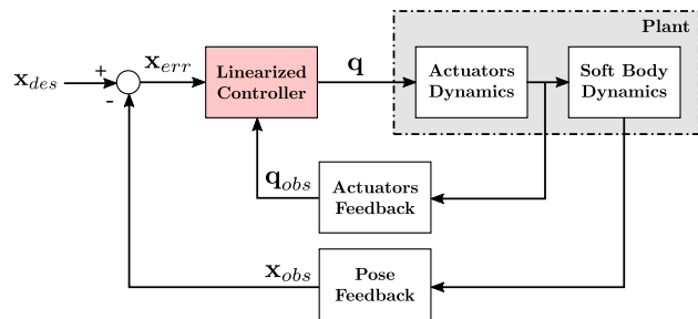
Figure 2. Block diagram representation of the proposed control system.
