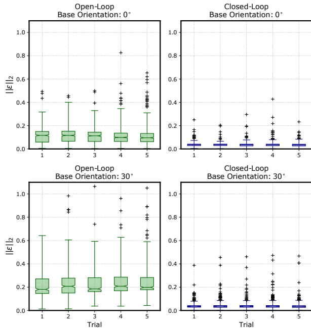
Figure 11. Box plot showing error distribution and variability over the 5 tests performed for each set of experiments for both closed-loop and open-loop, in the flat and pre-bent initial configuration.
