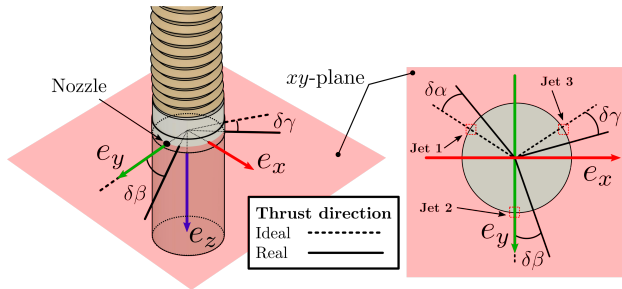
Figure 6. Waterjet actuation system: the force vectors generated by the jets lay on the tip xy -plane and are ideally spaced 120 degrees from each other. The parameters \delta\alpha, \delta\beta, \delta\gamma describe the jets misalignment, with respect to the ideal case, due to manufacturing imperfections.
