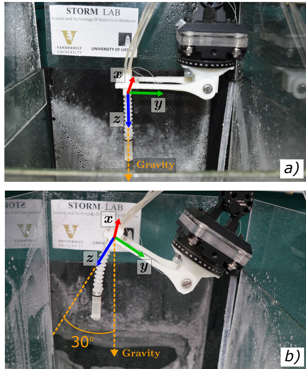
Figure 8. Starting configurations for the path following trials: a) initially straight and b) initially bent with respect to the direction of the gravity vector.
