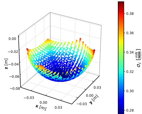
Figure 12. Stability test of the manipulator workspace for the initially straight case. The eigenvalues of the stiffness matrix remain positive throughout the entire actuation space.
