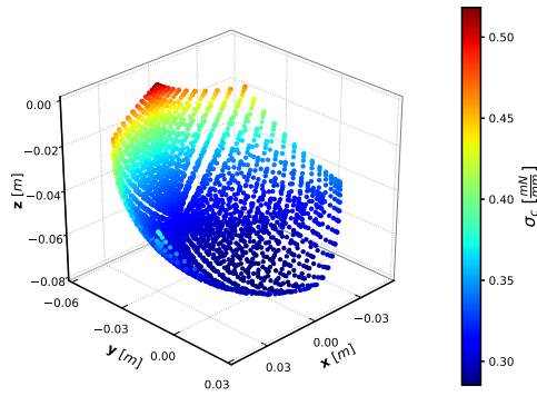
Figure 13. Stability test of the manipulator workspace for the initially bent case. The effective stiffness of the manipulator is not symmetric due to the rotation of the base frame. Similar to the initially straight case, the eigenvalues of the stiffness matrix remain positive throughout the entire actuation space.
