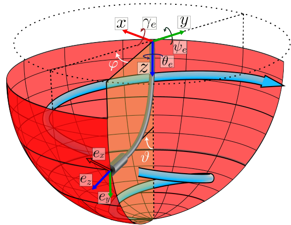
Figure 7. The HydroJet's workspace: the manipulator's tip can be maneuvered with two DoF by commanding \vartheta and \varphi .
