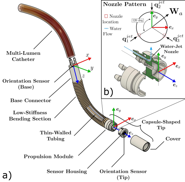
Figure 4. The HydroJet, a soft continuum endoscope manipulated via TFA that is used to experimentally validate the proposed control method, showing a) Exploded view of the continuum endoscope, and b) a detailed view of the locations of the water jet nozzles with respect to the tip frame.
