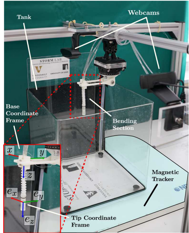
Figure 5. Experimental setup consisting of a magnetic tracker, two webcams and the HydroJet. At the bottom left corner, the base and tip reference frames are shown.
