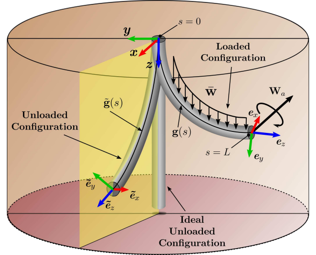
Figure 1. Soft continuum manipulator spatial configurations. In the ideal unloaded configuration the rod is perfectly straight. The unloaded configuration is pre-curved due to the existence of internal strain. The loaded configuration shows the rod bending under distributed and point loads.
