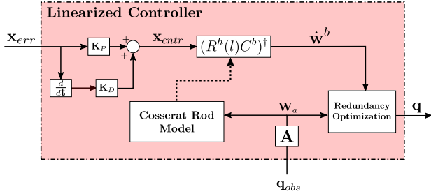
Figure 3. Block diagram detail of the linearized controller.
