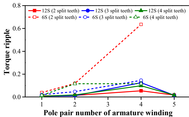
Figure 15. Torque ripples versus stator slot number, armature pole pair number, and split-tooth number when rotor slot number is selected as nN_s - P_a .
