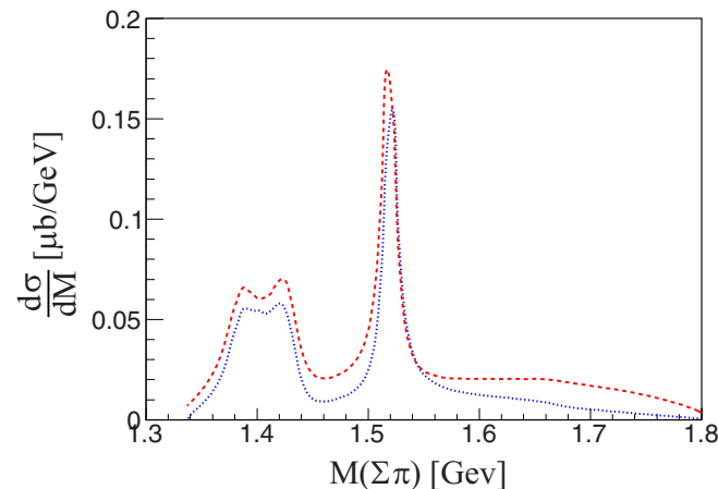
FIG. 8. Model predictions [11] to understand the difference in the K^{*0} background contributions to the decay of \Lambda^* into the two channels, \Sigma^+\pi^- and \Sigma^-\pi^+ , shown as short dashed and dotted curves, respectively. The predictions are shown as a function of \Sigma\pi invariant mass, M(\Sigma\pi) .
