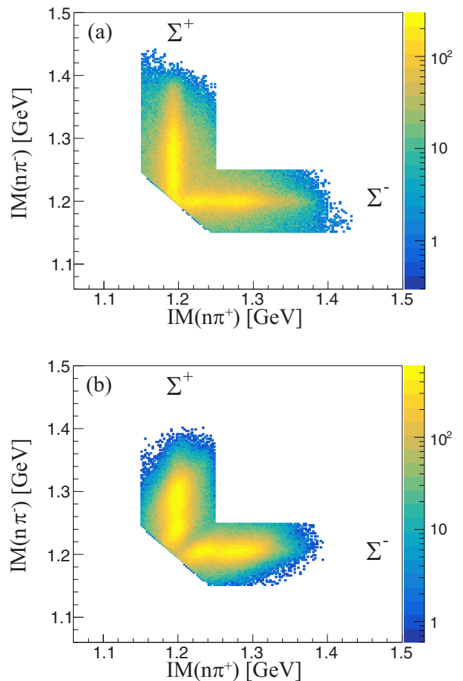
FIG. 9. The IM(n\pi^-) vs IM(n\pi^+) distributions for data in (a) and simulation in (b) with the vertical and horizontal strips reflecting \Sigma^+ and \Sigma^- , respectively, are shown.
