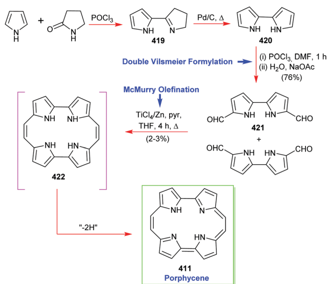
Scheme 58 Vogel's synthesis of porphycene.
