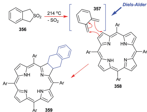
Scheme 49 Exemplary cycloaddition reaction involving porphyrins. Cavaleiro and coworkers' use of meso -tetraarylporphyrins 358 as dienophile in a Diels–Alder reaction with ortho -benzoquinodimethane 357 to give chlorin 359 (plus other products).
