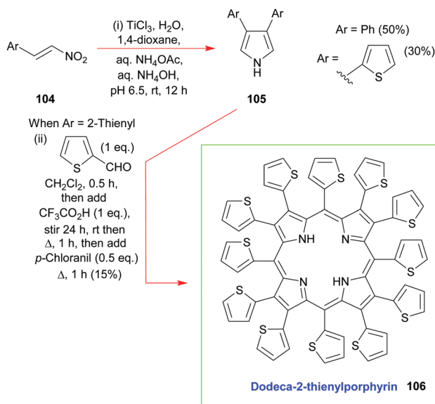
Scheme 14 Ono's Ti(III)-mediated synthesis of 3,4-diaryl- and 3,4-diheteroaryl-pyrroles and the subsequent use of these intermediates in the synthesis of dodeca-2-thienylporphyrin 106 .
