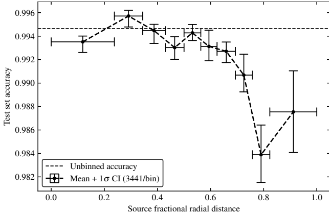
Figure 10. Class-balanced accuracy evaluated on the test set as a function of detector position. We use a series of concentric radial bins, chosen to contain equal numbers of sources for uniform statistics. We scale the radius through by the detector size to give a relative picture of performance. The drop in performance at large radial distances is primarily caused by the extreme optical distortion present in the early GOTO prototype, and only a minor drop of 1% in accuracy in these challenging conditions demonstrates the very robust performance of our classifier. With the design-specification GOTO optics, we anticipate this curve will be level within error.
