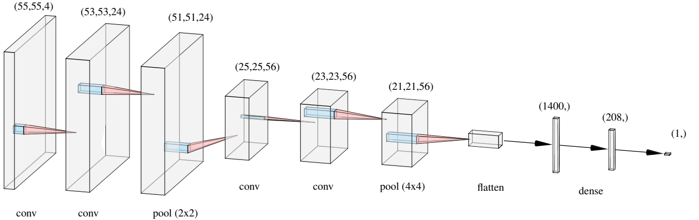
Figure 4. Block schematic of the optimal neural network architecture found by hyperparameter optimisation in Section 3.1. Each block here represents a 3D image tensor, either as input to the network, or the product of a convolution operation generating an ‘activation map’. Classification is performed using the scalar output of the neural network. Directly above each 3D tensor block the dimensions in pixels are shown, along with the operation that generates the next block below it represented by the coloured arrow. Not illustrated for clarity here are the dropout masks applied between each layer and the activation layers. Base figure produced with NNSVG (LeNail 2019).
