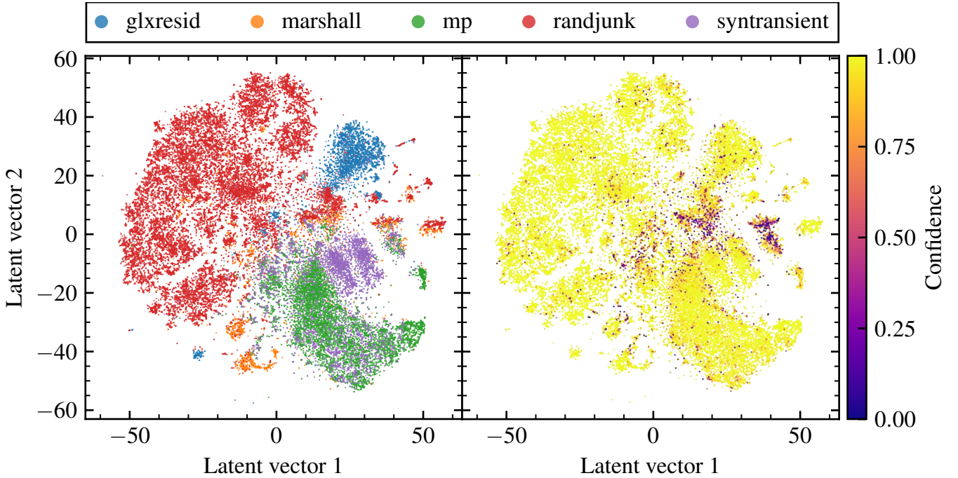
Figure 8. Example class-clustering (left) and confidence (right) maps generated from the classifier’s test set. Each colour in the left panel represents a specific sub-class of detections, where colour on the right represents classifier confidence. The top legend gives the classes corresponding to each colour in the left panel. Regions of low confidence in the right panel tend to correspond to cluster boundaries in the left, where there is more uncertainty about which class each example belongs to.
