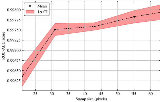
Figure 5. Classifier performance on the test set of a 330,000 example training set as a function of input stamp size. Each point is the average of 3 independent training runs on the same input training set, with the shaded region representing the 1\sigma confidence interval.
