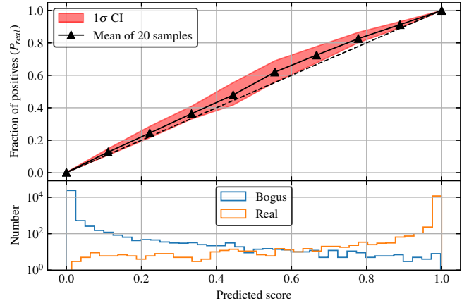
Figure 12. Top panel: classifier calibration curve, illustrating how well the classifier’s output score corresponds to probability. The mean of 20 samples and the 1\sigma confidence interval are plotted to show that individual draws from the posterior remain well-calibrated. Bottom panel: Score distribution for both real and bogus examples – with the relative scarcity of examples with 0.2 < RB < 0.8 accounting for the greater uncertainty in calibration.
