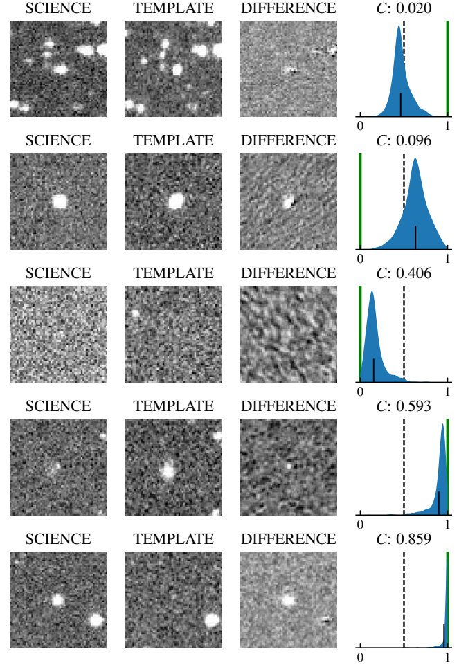
Figure 7. A selection of example posteriors, taken from real GOTO data. The majority of predictions are highly confident, so we select examples of increasing confidence score (C) to display here. Plotted here is a Gaussian kernel-density estimate constructed from 500 posterior samples. The green line indicates the correct label for each candidate, with the black line indicating the mean of the distribution. The dashed line indicates P_{\text{real}} = 0.5
