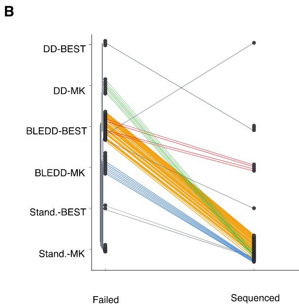
Fig. 2. Success rates of high-throughput library preparation from Atlantic cod bones. (A) Schematic of libraries generated for all archaeological sites (yellow, sequenced; gray, processed but not sequenced library) divided into groups according to DNA extraction and library preparation protocols utilized. Note that the number of libraries can be higher than the number of specimens (Ind) due to multiple treatments. DD = double digestion extraction protocol, BLEDD = bleach treatment combined with double digestion extraction protocol, MK = Meyer-Kircher library preparation protocol, BEST = single tube library preparation protocol. (B) Treatment overview for samples processed using multiple library and extraction treatment combinations ( n = 73 ). Treatments are abbreviated according to Fig. 2A, and different treatment combinations per sample are indicated by connecting lines and colored according to treatment combination. (C) Sensitivity analysis: density distribution of significant factors (site, DNA extraction and library preparation protocols) following iterative ( i = 100 ) logistic regression (library outcome \sim extraction protocol + library protocol + site + bone element + (1 | Sample)), using randomly resampled data. (For interpretation of the references to color in this figure legend, the reader is referred to the Web version of this article.)
