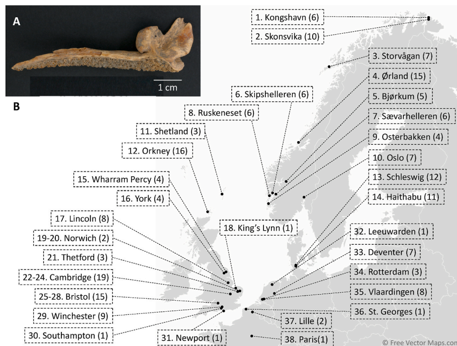
Fig. 1. Archaeological Atlantic cod bones. (A) Archaeological Atlantic cod jawbone (premaxilla) from the site of Orkney Quooygrew (1000–1200 CE). (B) Locations of fish bone specimens ( n = 204 ) from 38 archaeological sites. Bones from Norwich, Cambridge and Bristol were obtained from distinct, individually numbered archaeological sites (see Table 1).
